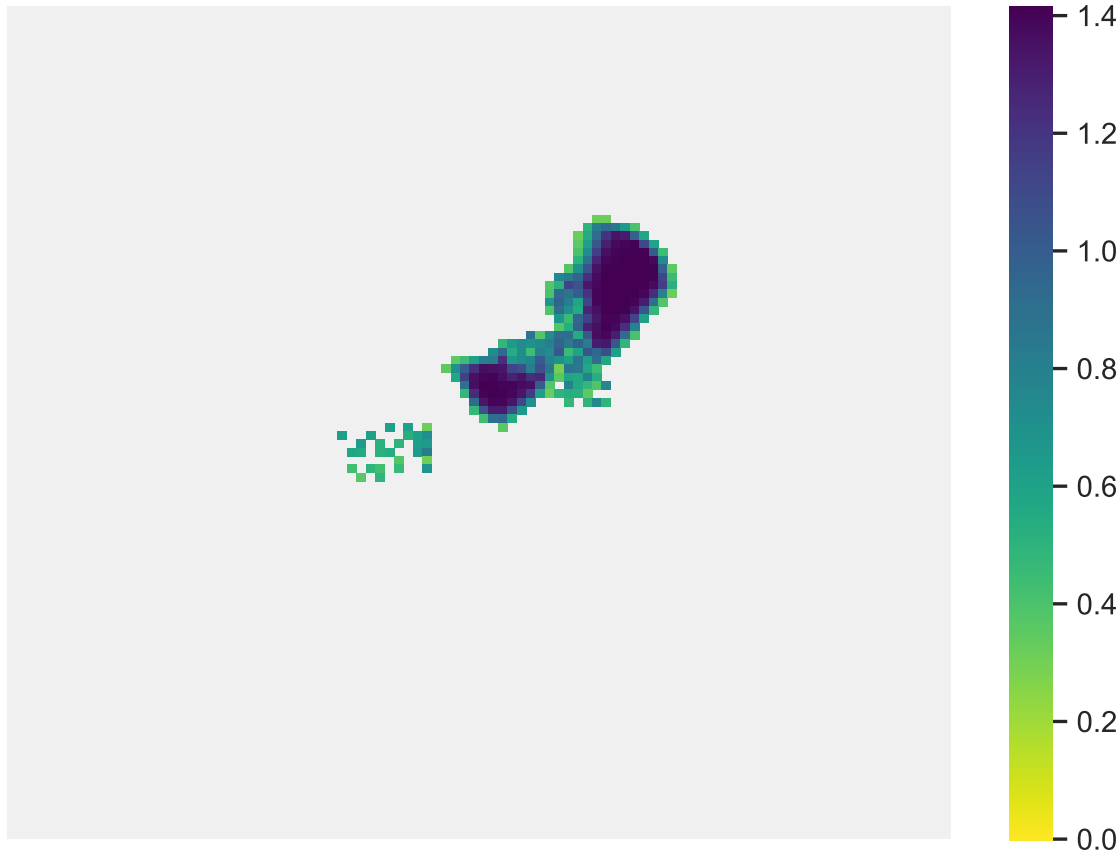
Sp. 4 (pop. size: 3462, range size: 311)
