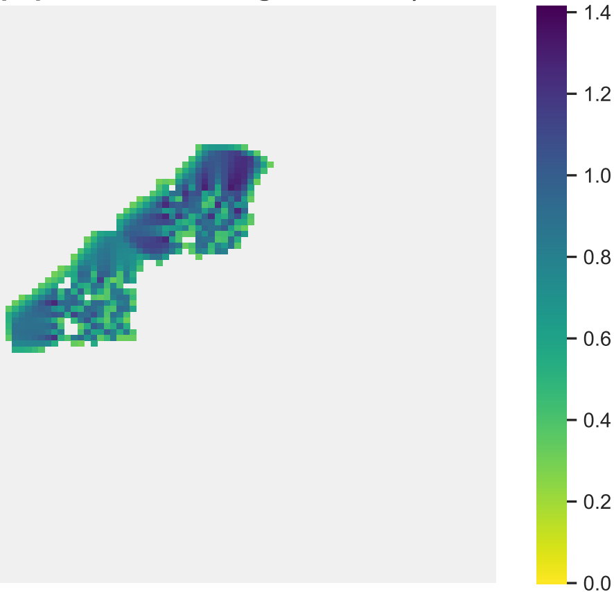
Sp. 8 (pop. size: 3559, range size: 583)
