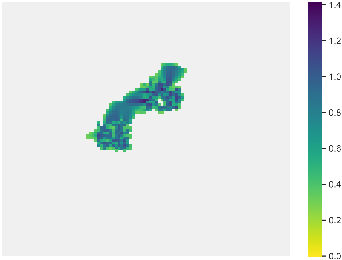
Sp. 2 (pop. size: 2581, range size: 478)
