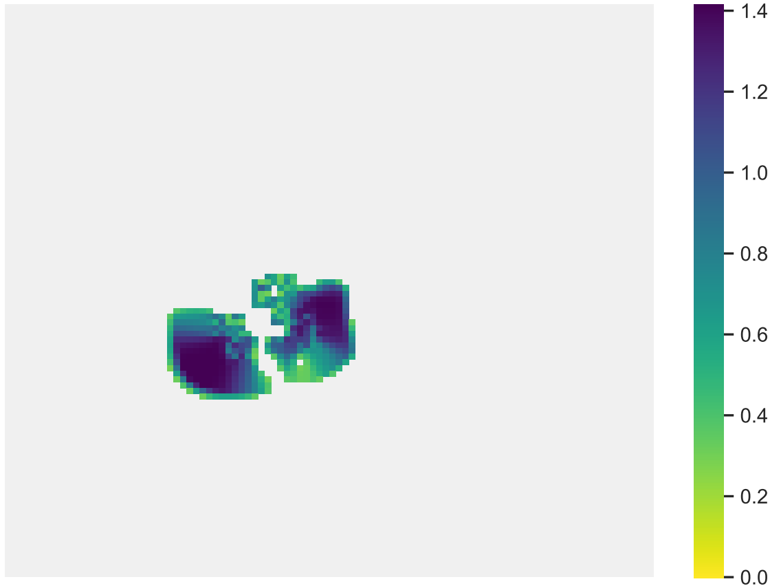
Sp. 6 (pop. size: 4481, range size: 426)
