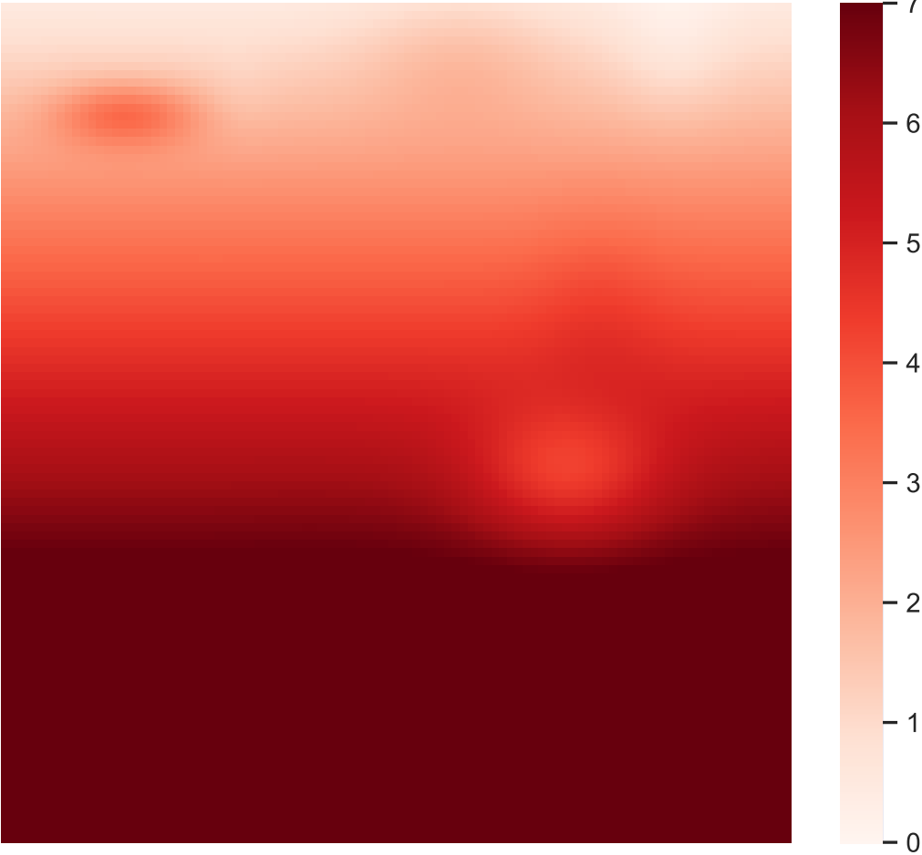
Mean annual temperature (mean anomaly: 5.42)
