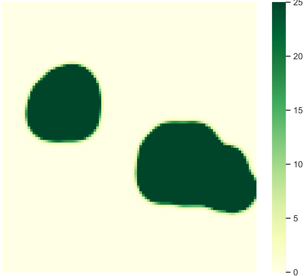
Mean population density (mean: 4.9)
