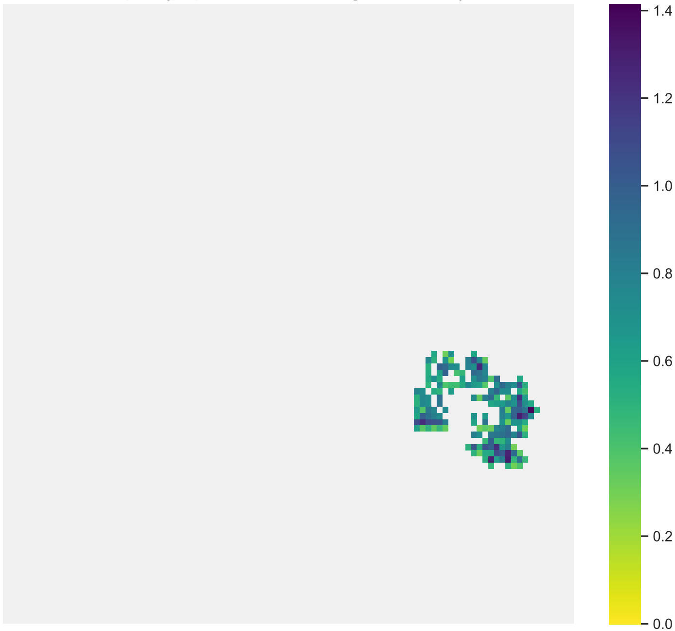
Sp. 4 (pop. size: 1014, range size: 187)
