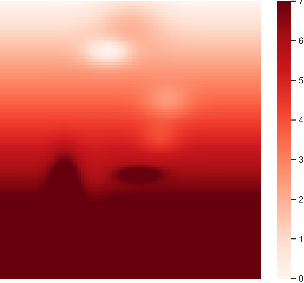
Mean annual temperature (mean anomaly: 4.99)
