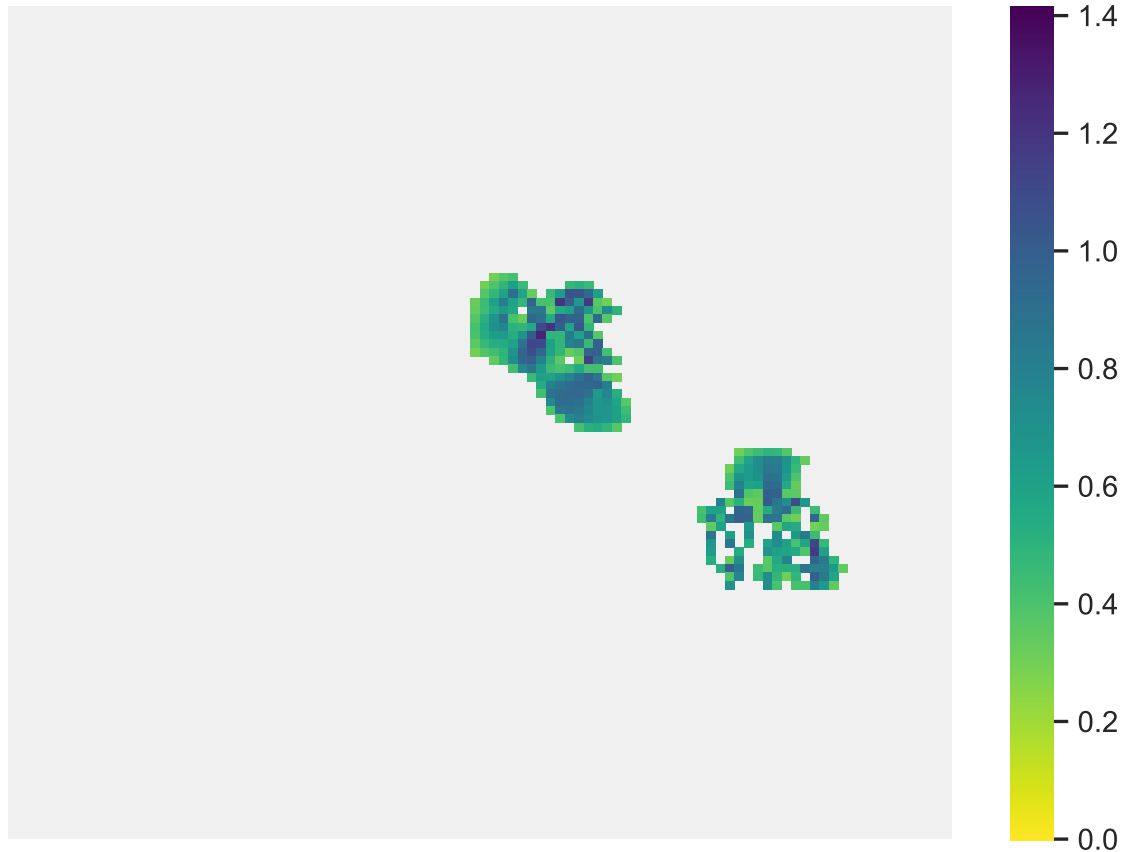
Sp. 8 (pop. size: 1552, range size: 358)
