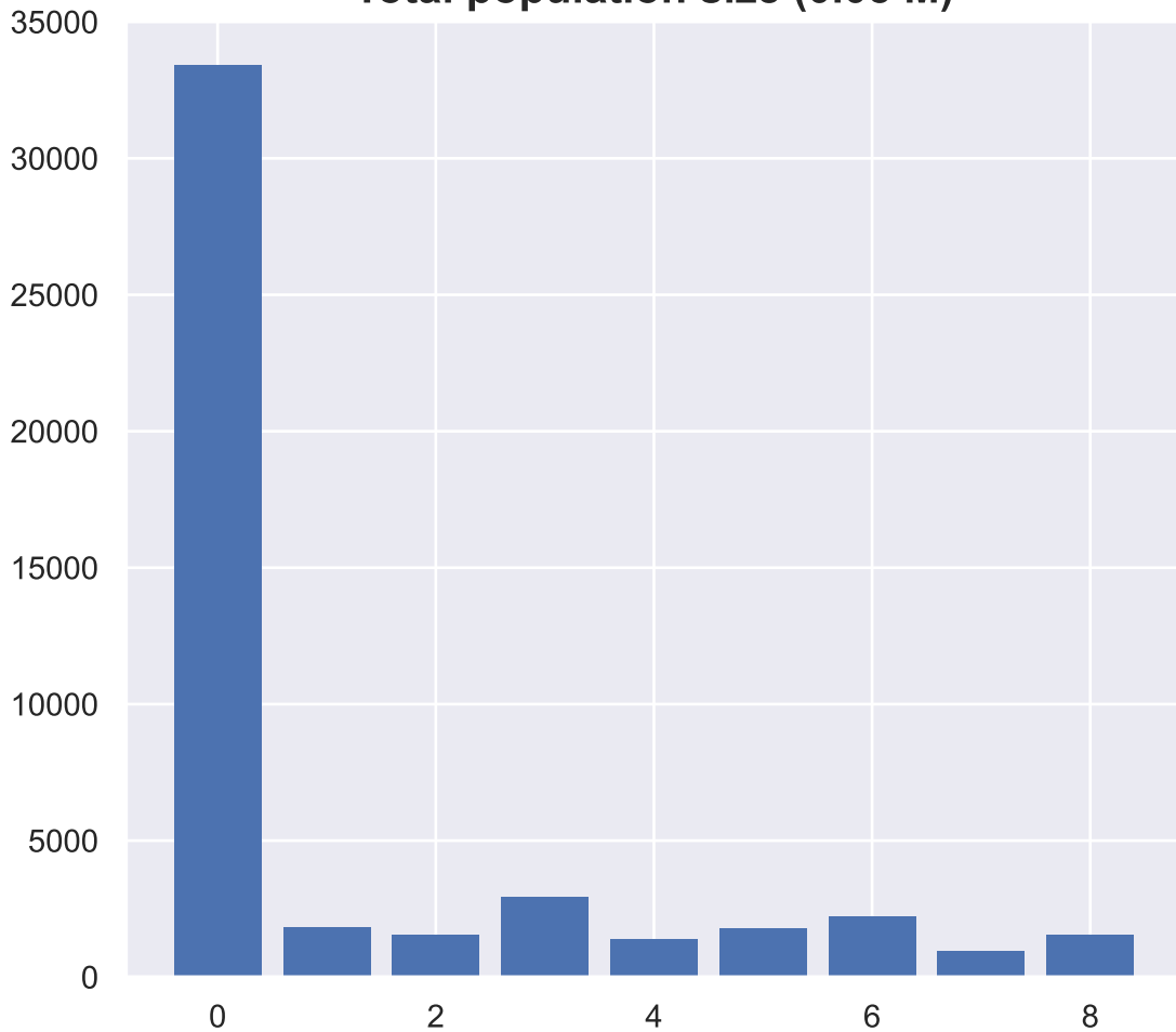
Total population size (0.05 M)
