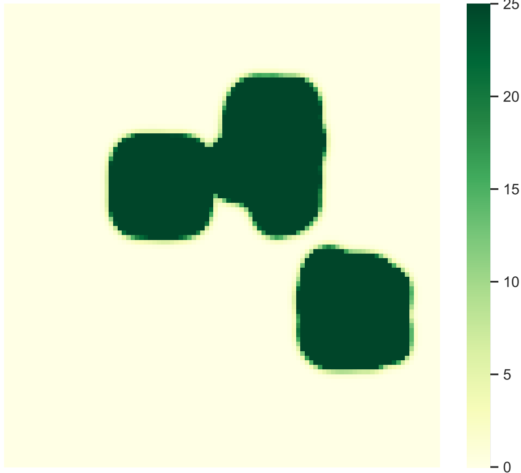
Mean population density (mean: 4.8)
