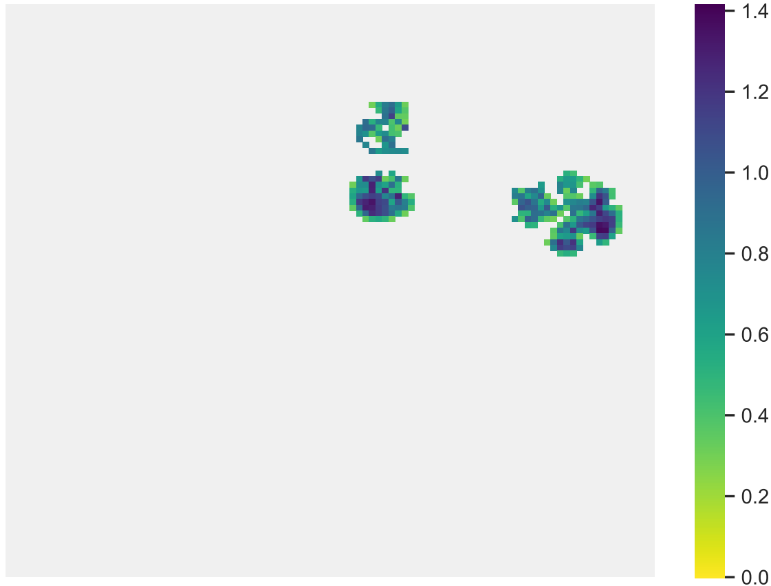
Sp. 5 (pop. size: 1690, range size: 266)
