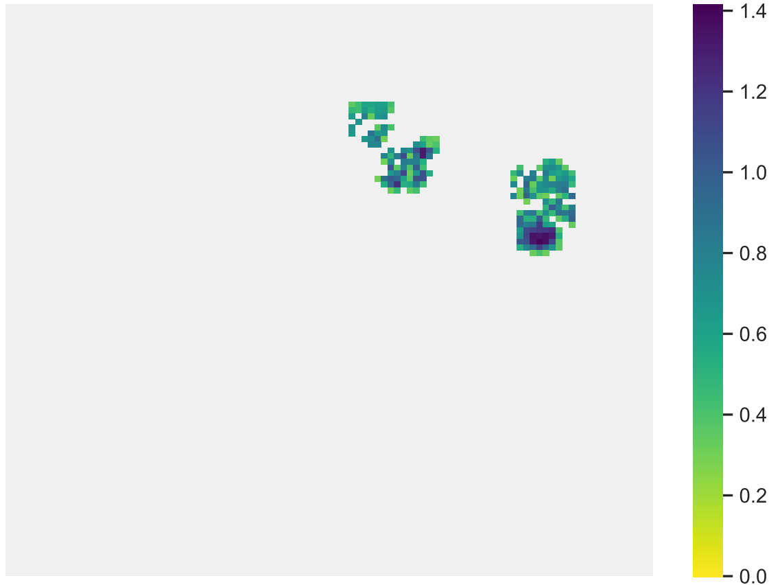
Sp. 6 (pop. size: 1169, range size: 210)
