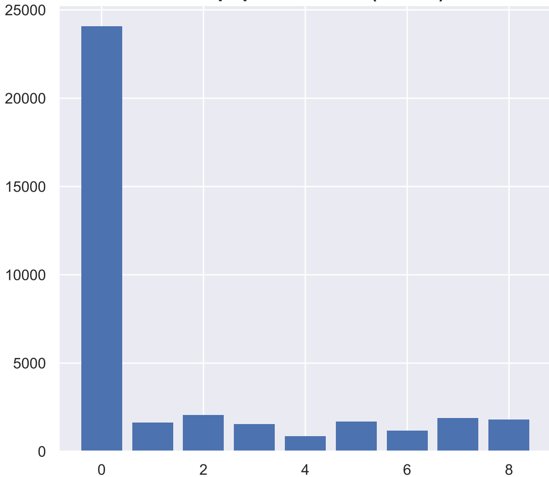
Total population size (0.04 M)
