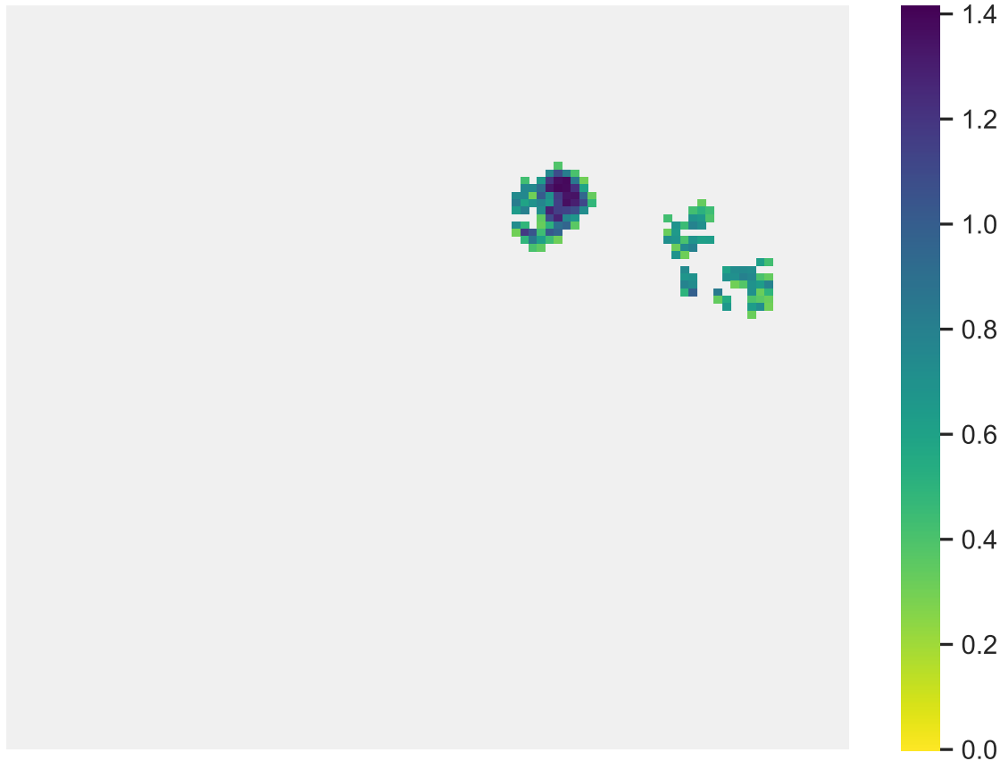
Sp. 4 (pop. size: 848, range size: 136)
