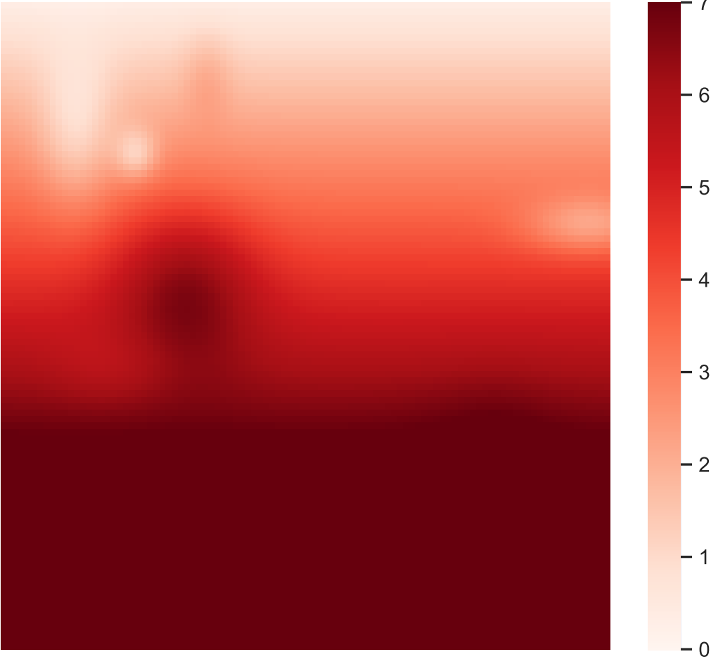
Mean annual temperature (mean anomaly: 5.36)
