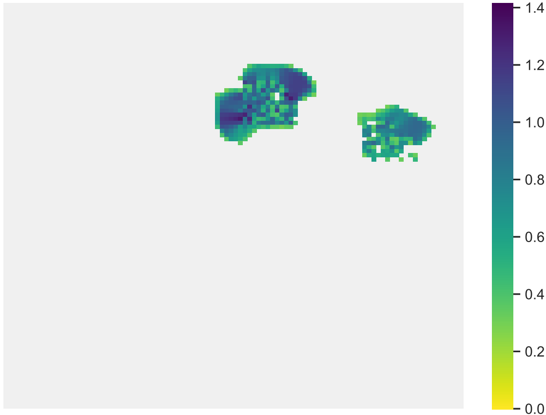
Sp. 2 (pop. size: 2551, range size: 443)
