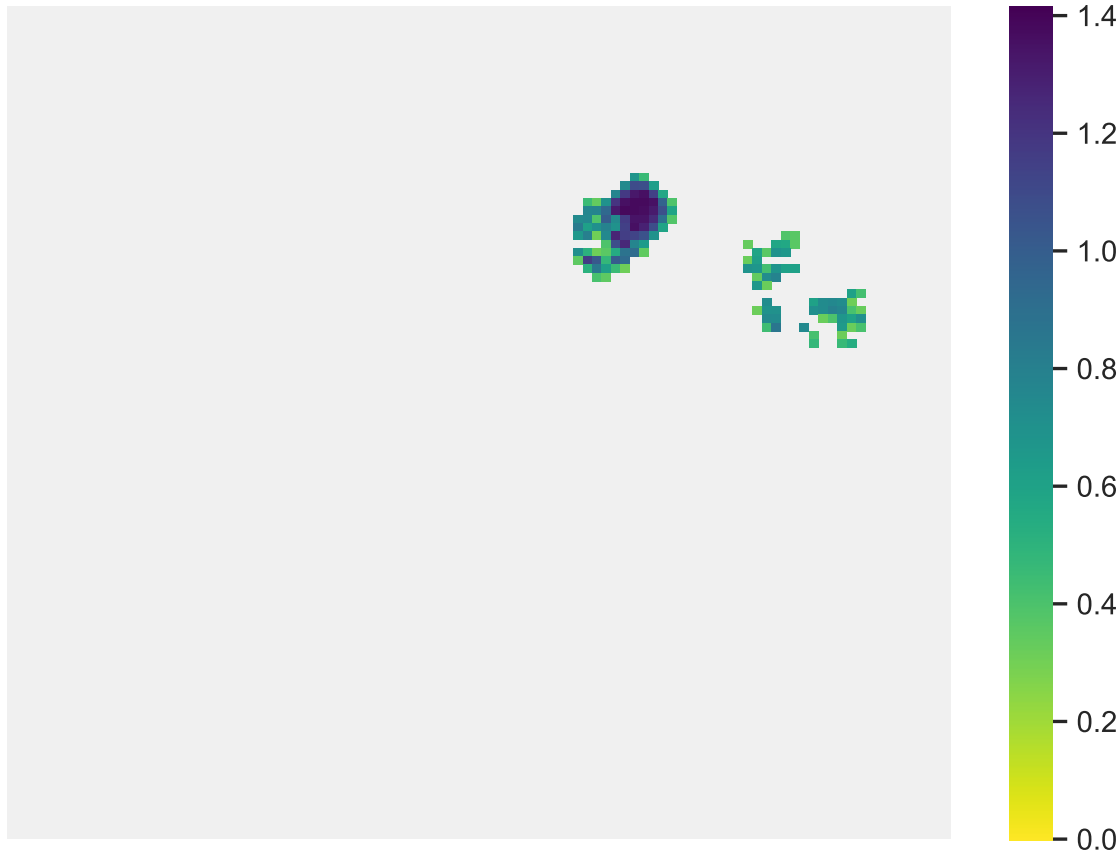
Sp. 4 (pop. size: 1019, range size: 146)
