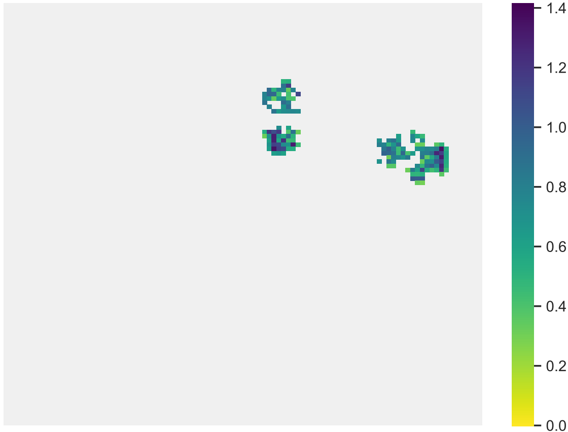
Sp. 5 (pop. size: 985, range size: 165)
