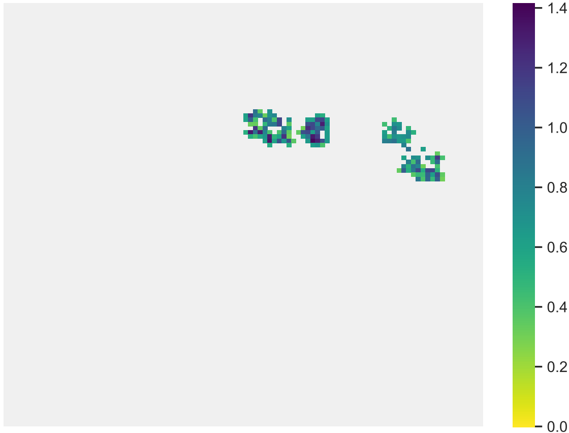
Sp. 3 (pop. size: 992, range size: 162)
