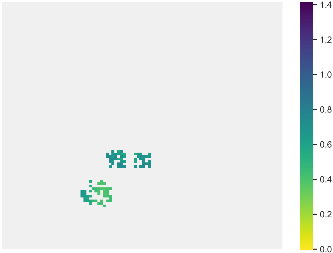
Sp. 3 (pop. size: 329, range size: 100)
