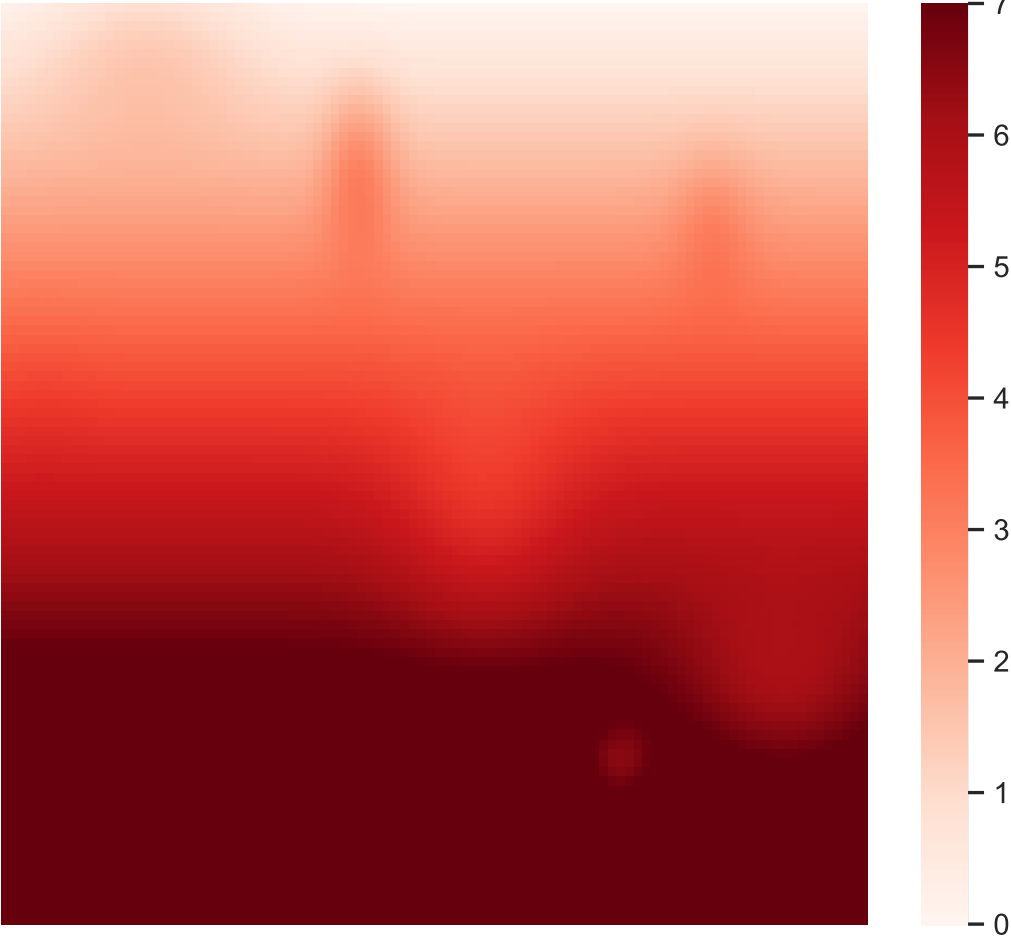
Mean annual temperature (mean anomaly: 4.94)
