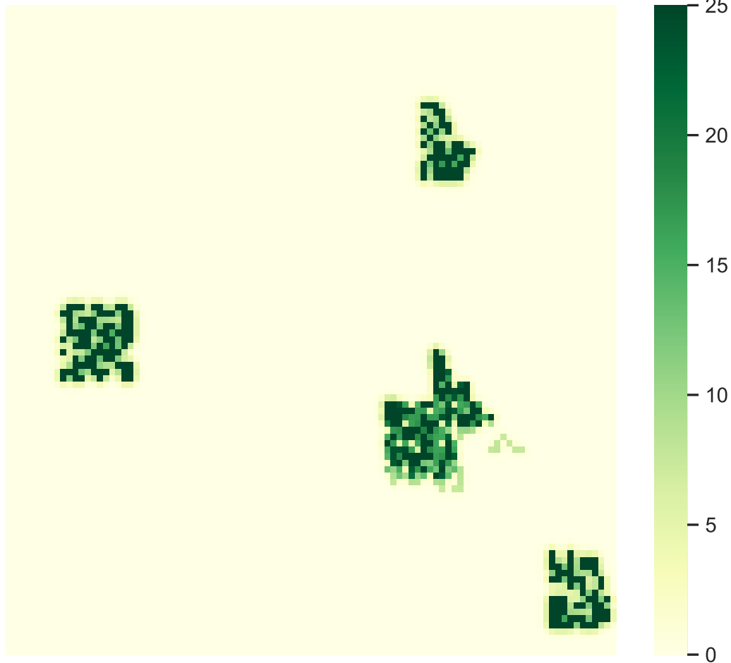
Mean population density (mean: 1.0)
