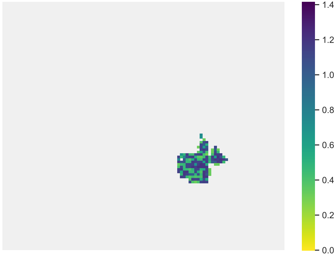
Sp. 2 (pop. size: 1395, range size: 175)
