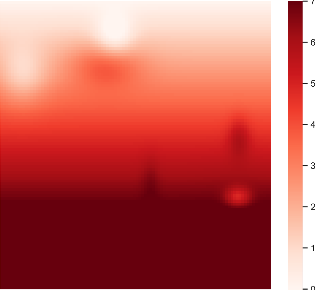
Mean annual temperature (mean anomaly: 5.03)
