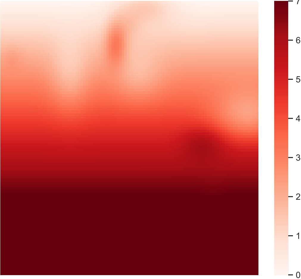
Mean annual temperature (mean anomaly: 4.92)
