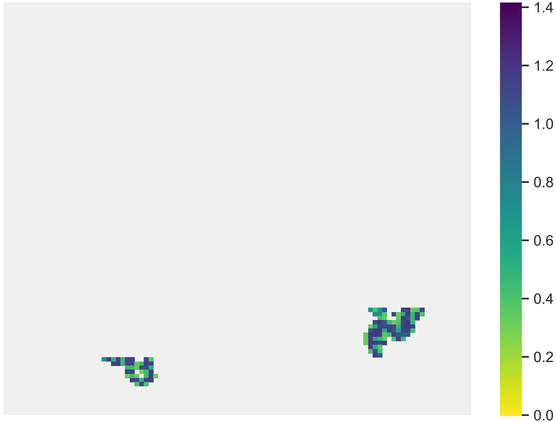
Sp. 2 (pop. size: 1027, range size: 129)
