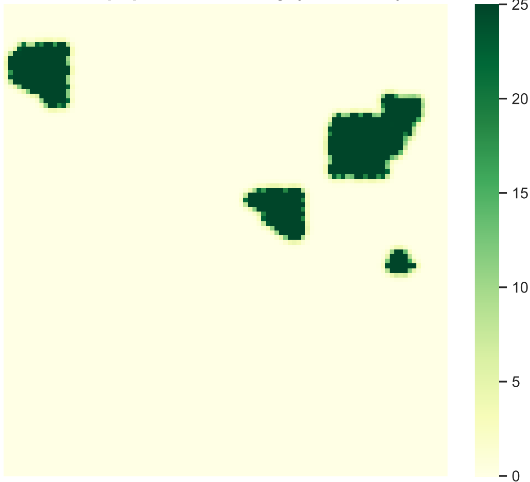
Mean population density (mean: 1.4)
