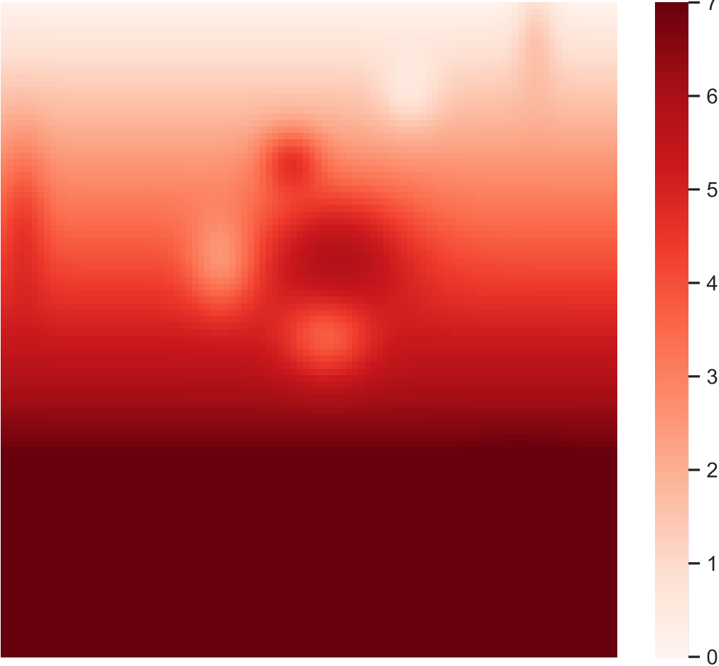
Mean annual temperature (mean anomaly: 5.18)
