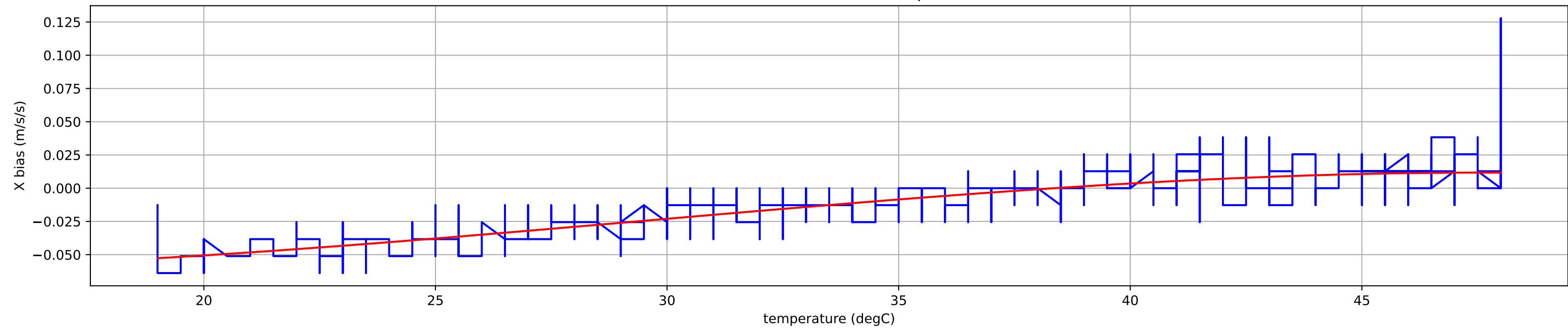
Accel 0 (4259850) Bias vs Temperature
