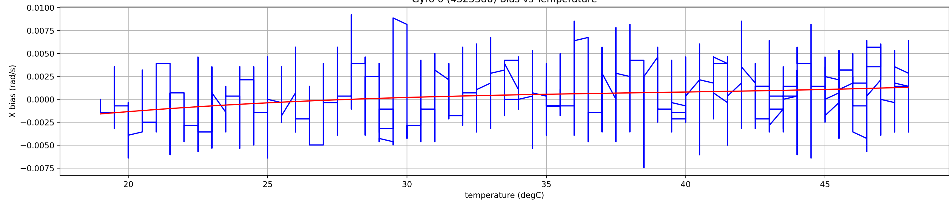
Gyro 0 (4325386) Bias vs Temperature
