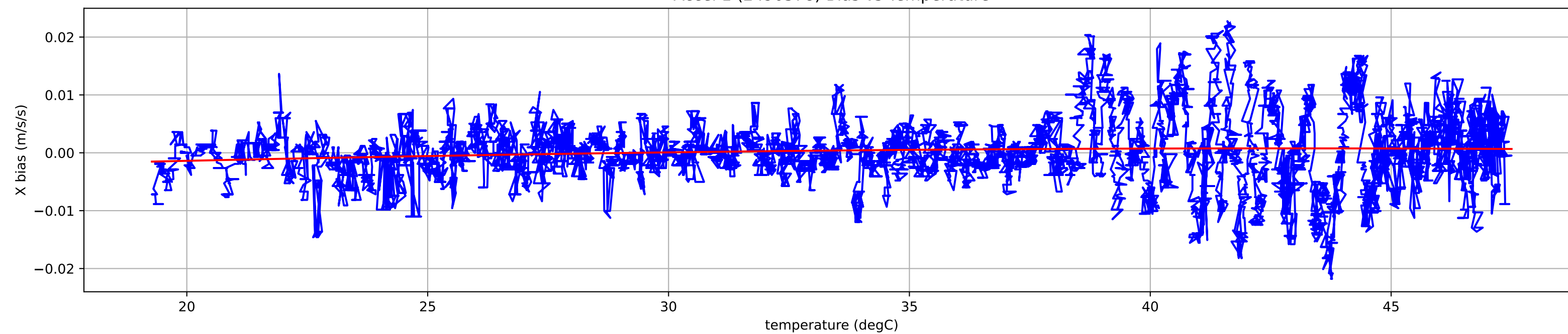
Accel 1 (2490378) Bias vs Temperature
