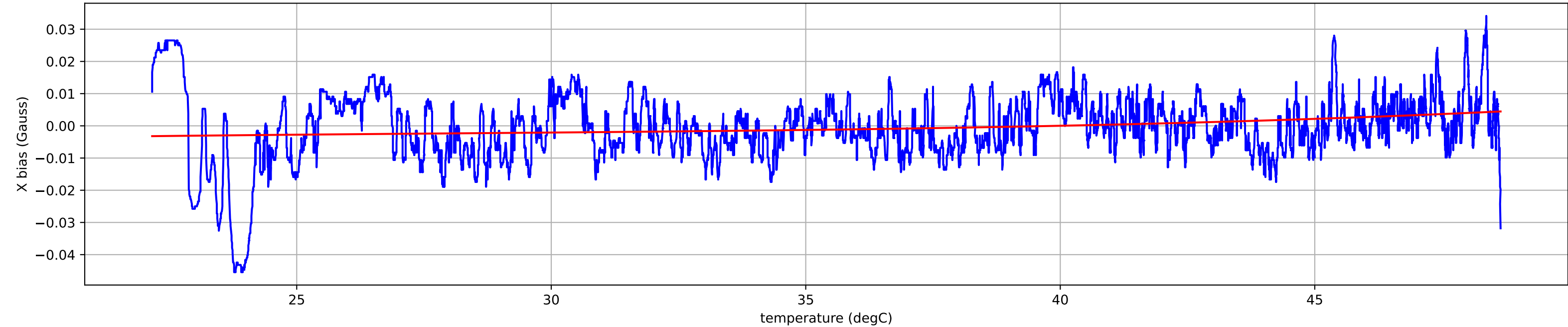
Mag 0 (0) Bias vs Temperature
