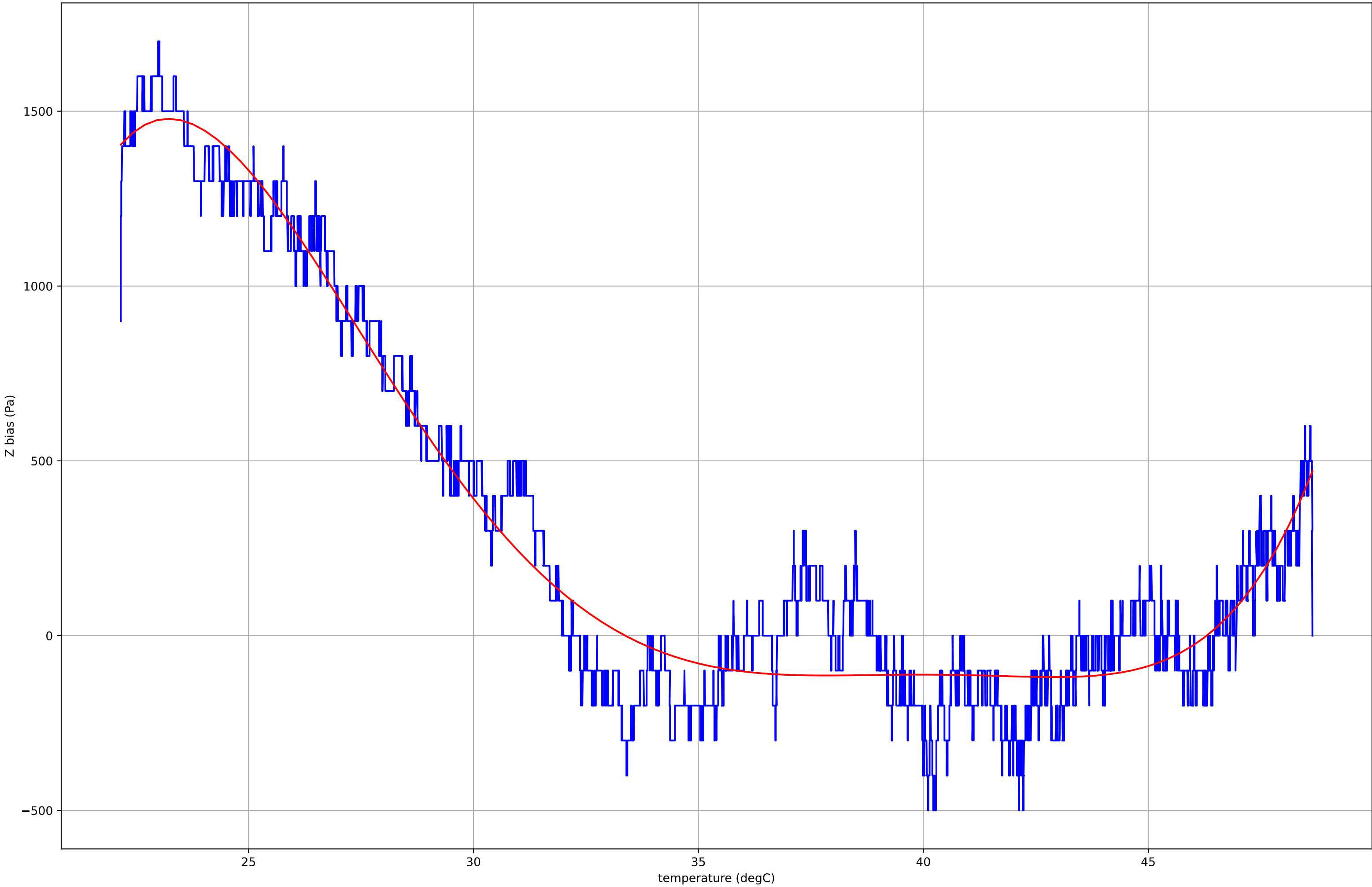
Baro 0 (4028193) Bias vs Temperature
