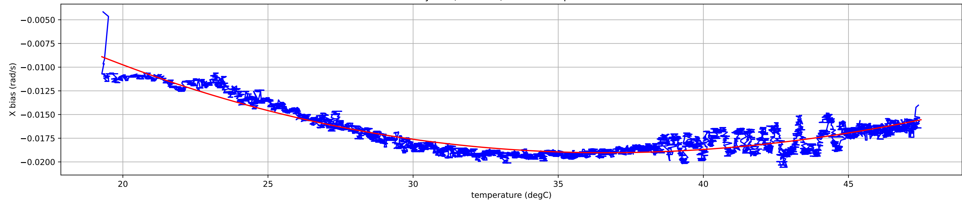
Gyro 1 (2490378) Bias vs Temperature
