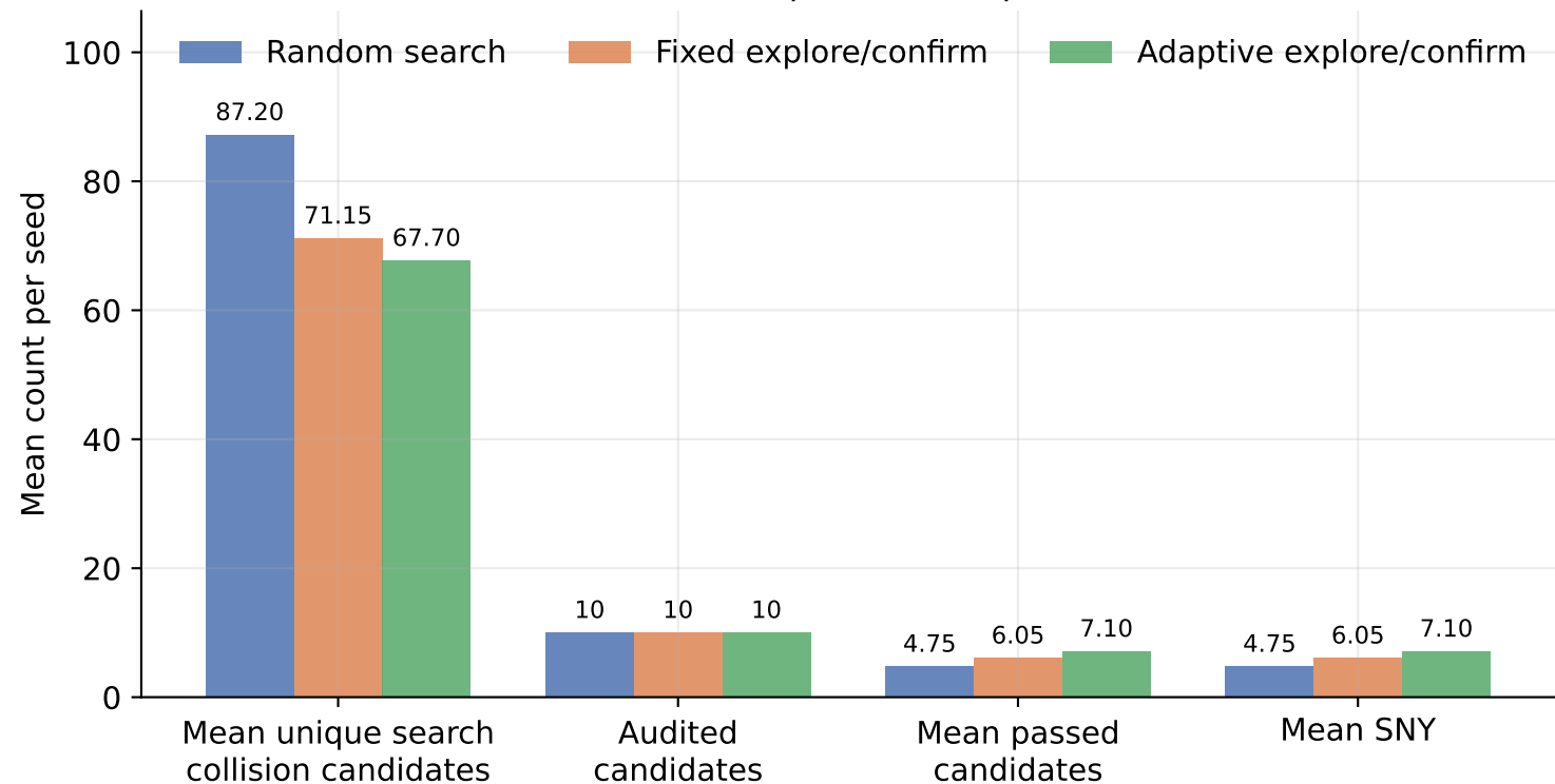
Search-to-audit funnel (descriptive, mean per seed over 20 seeds)
