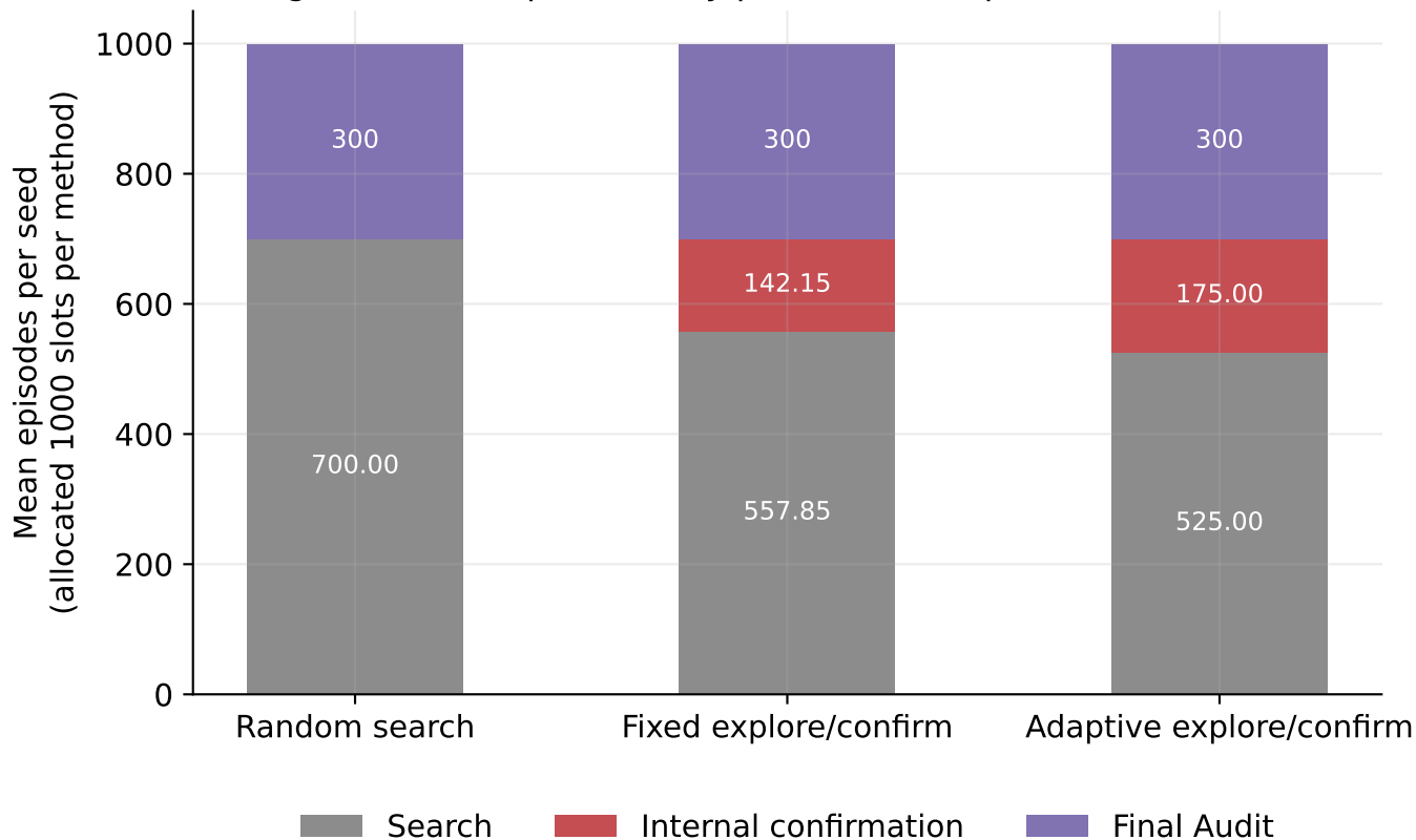
Budget allocation per seed by phase (search pool 700 + audit 300)
