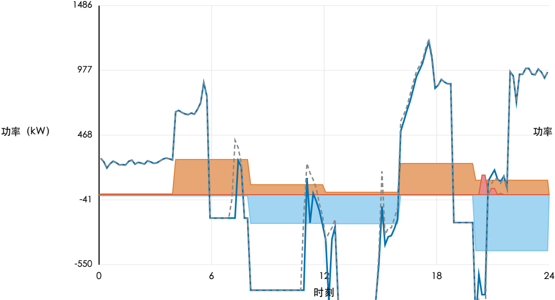
2025-09-23 (当日紧急购电 419 kWh)
