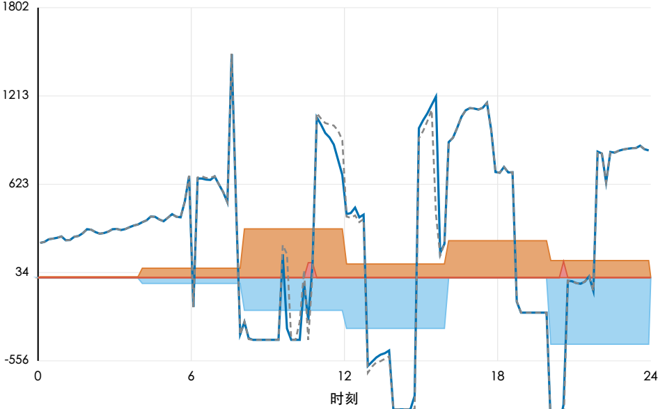
2025-12-21 (当日紧急购电 308 kWh)
