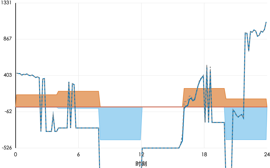
2025-06-21 (当日紧急购电 0 kWh)
