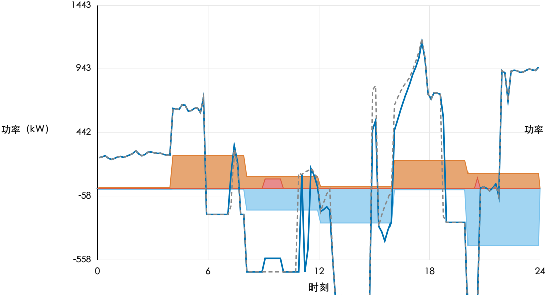
2025-03-20 (当日紧急购电 560 kWh)
