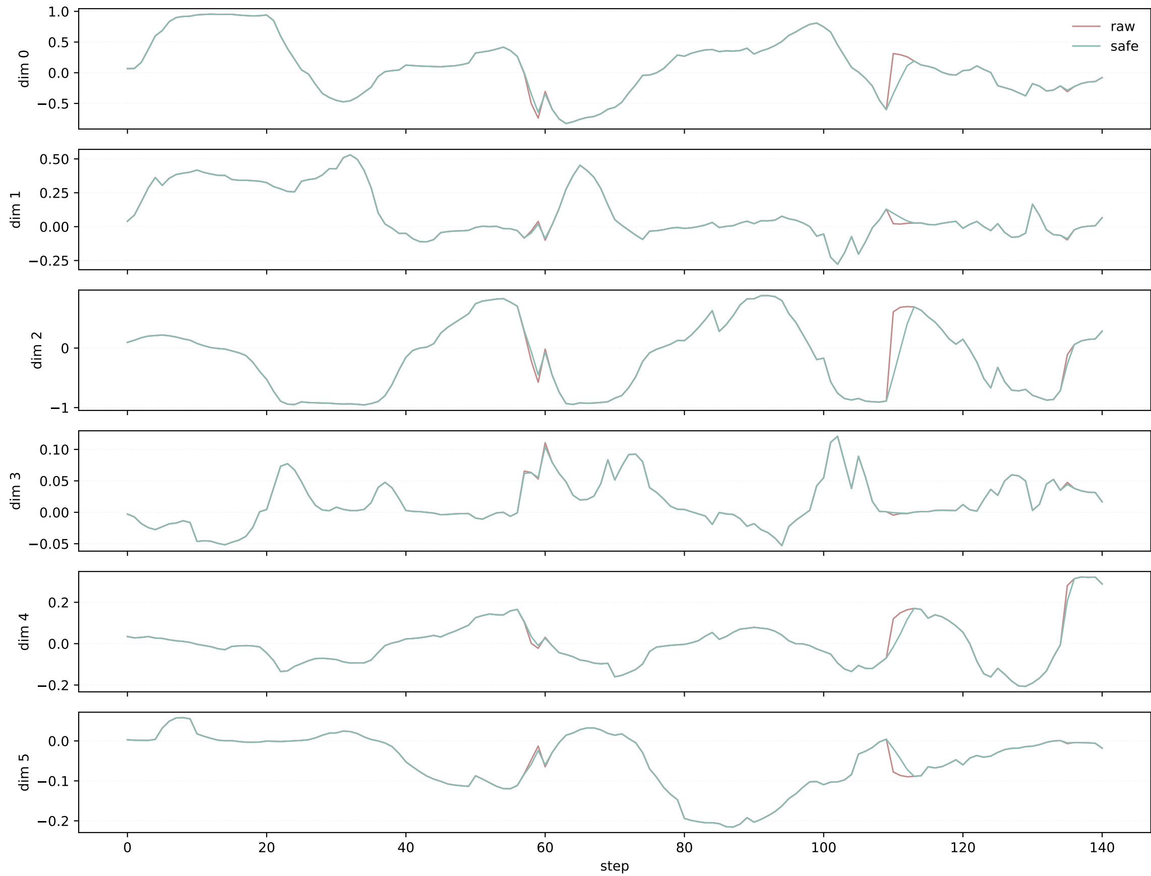
Raw vs Safe Motion Actions [actions.npy]
