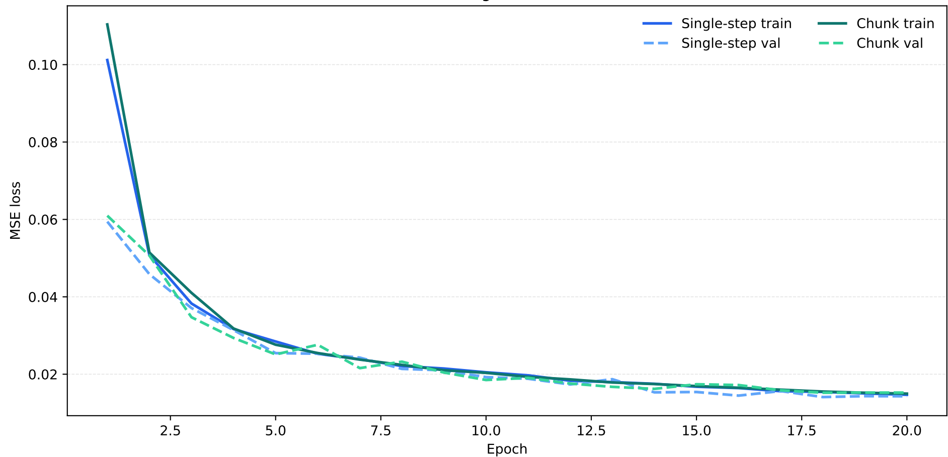
Training loss curves
