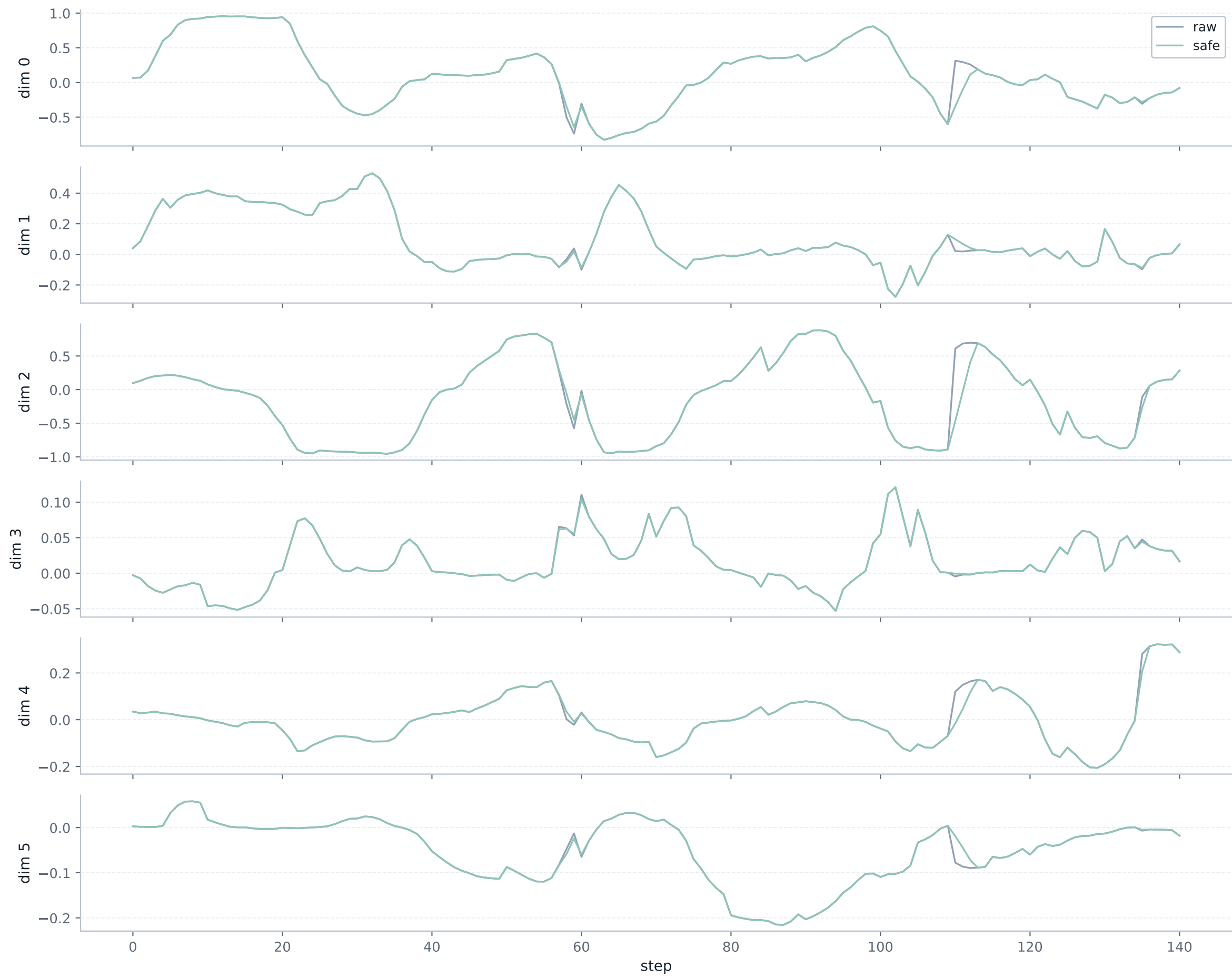
Raw vs Safe Motion Actions [actions.npy]
