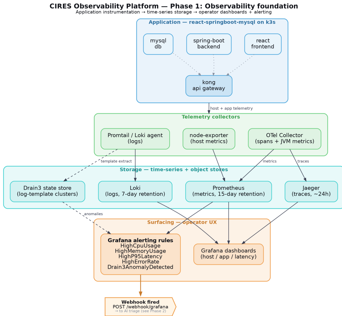
Figure 4.2. Phase 1 — observability foundation. Application instrumentation (Spring Boot, Kong, MySQL, k3s) flows into collectors (Prometheus scrape, Promtail, OTEL Collector) and into storage (Prometheus TSDB, Loki, Jaeger). Grafana surfaces the data and routes alerts through the unified-alerting webhook contact point.
