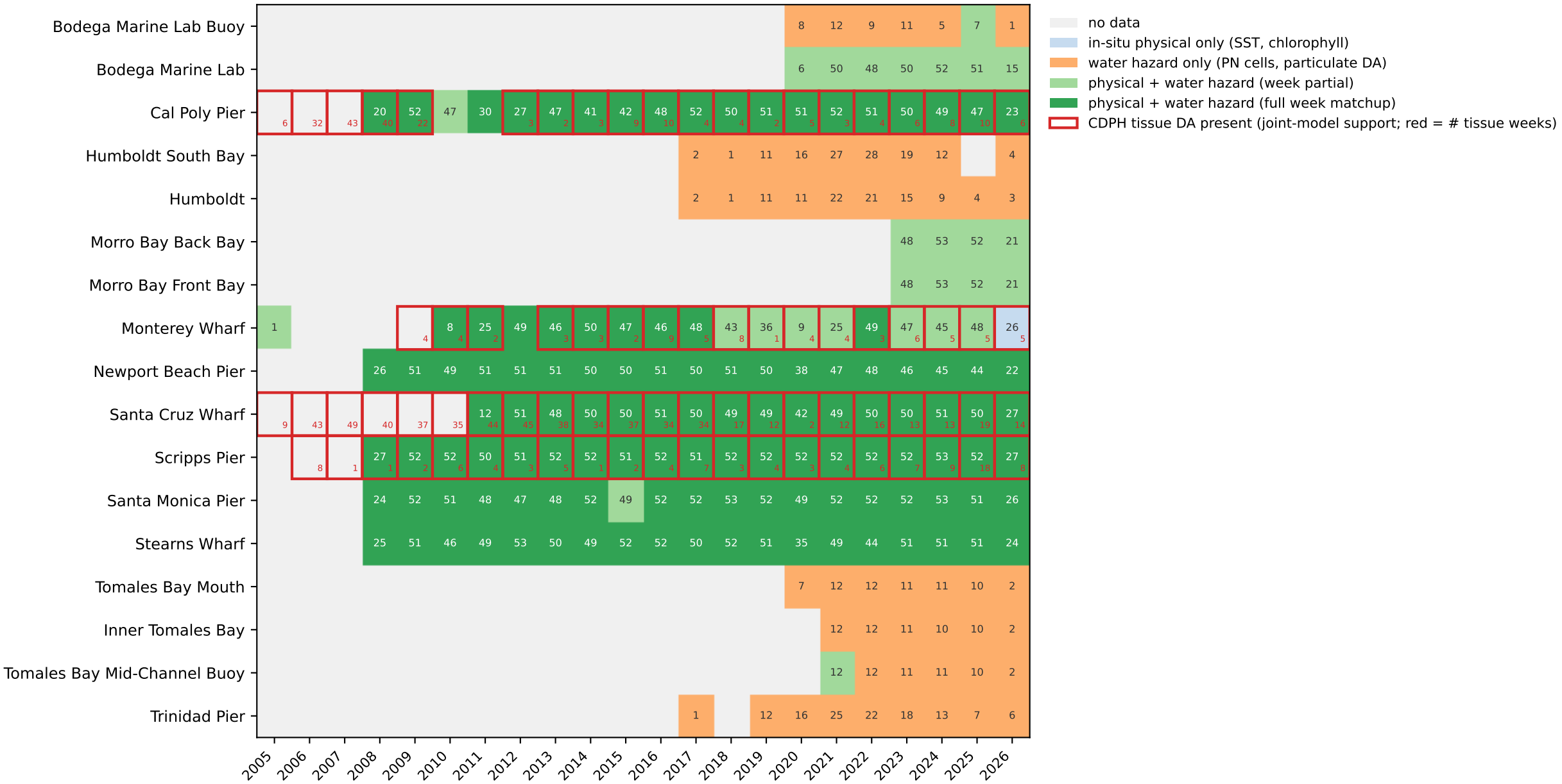
HAB data coverage by site x year background = calHABMAP (centre # = weekly rows); red border = CDPH tissue DA
