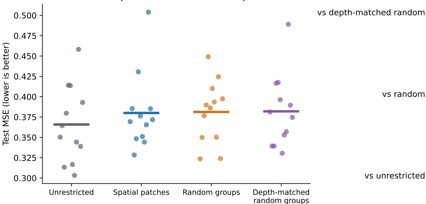
A. Main comparison: 12 matched fits per model
