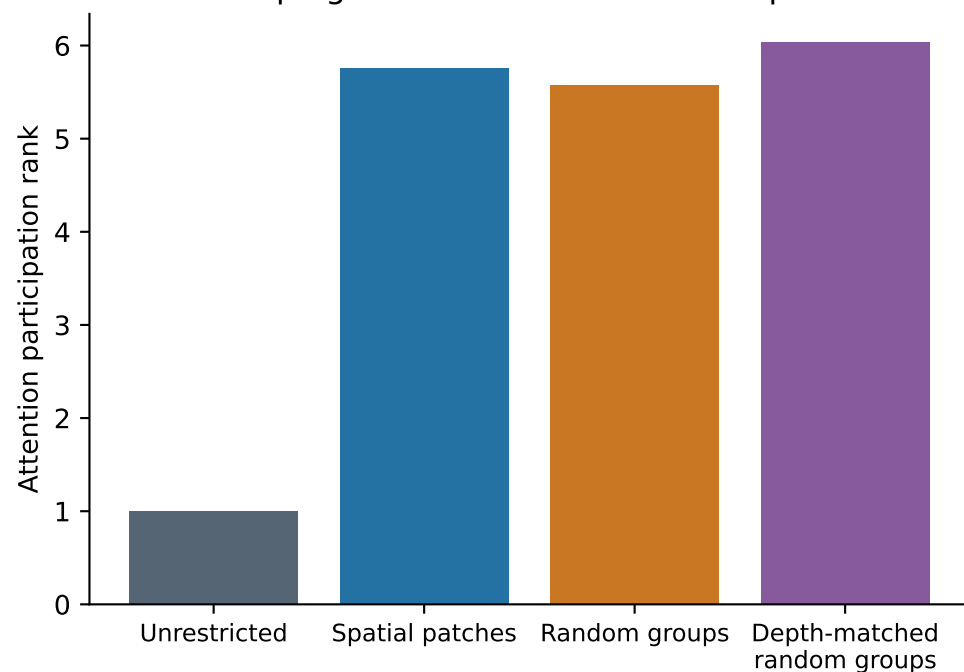
C. Grouping creates distinct attention patterns
