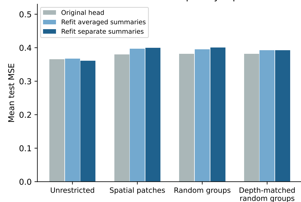
D. Frozen-encoder output-layer probe
