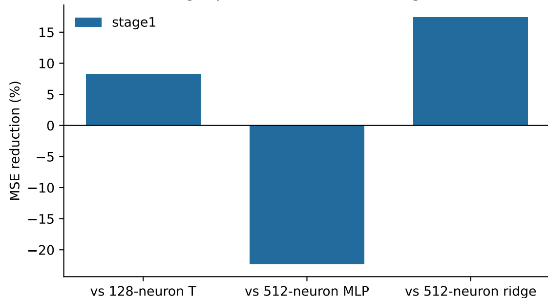
Larger-panel transformer mean gains
