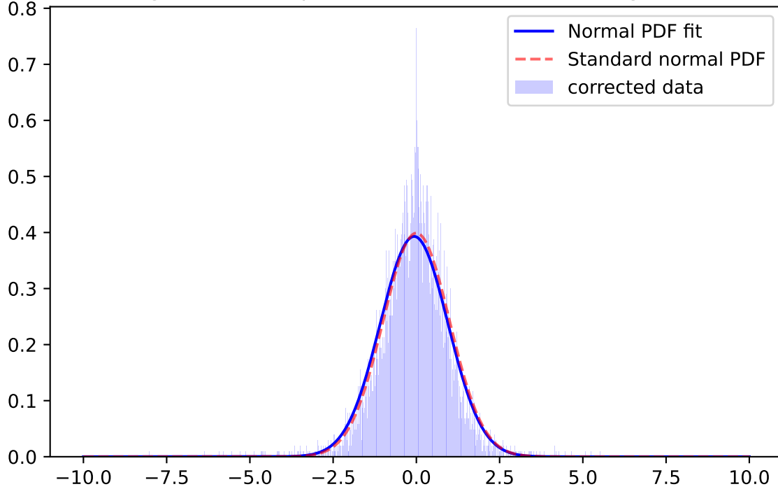
Whiten Signal, z-band, \mu=-0.0676 \sigma=1.0150 ; for mag=[18.0; 18.5]
