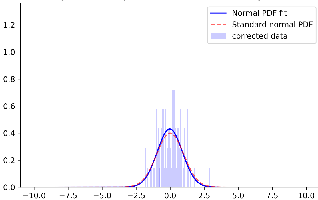
Whiten Signal, r-band, \mu=-0.0310 \sigma=0.9950 ; for mag=[18.0; 18.5]
