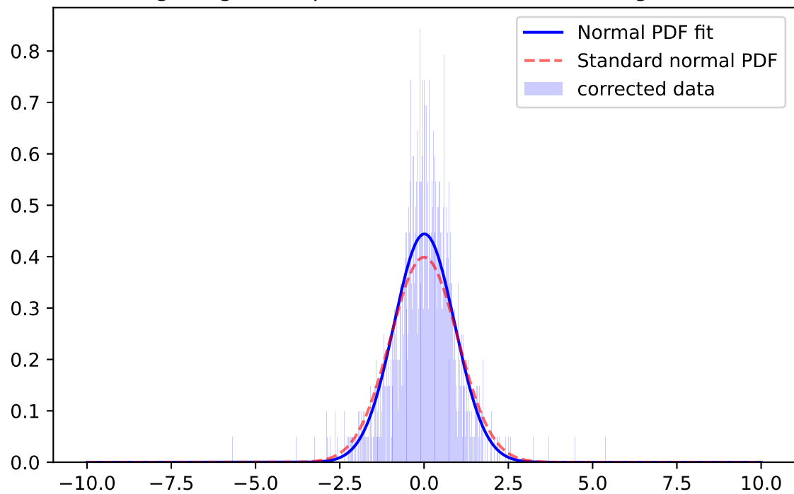
Whiten Signal, i-band, \mu=-0.0258 \sigma=1.2067 ; for mag=[18.0; 18.5]
