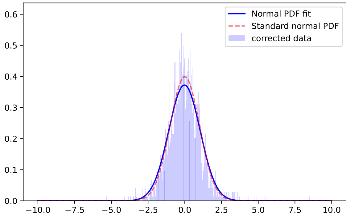
Whiten Signal, y-band, \mu=-0.0250 \sigma=1.0715 ; for mag=[18.0; 18.5]
