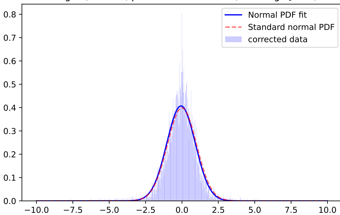
Whiten Signal, z-band, \mu=-0.0650 \sigma=0.9801 ; for mag=[18.0; 18.5]
