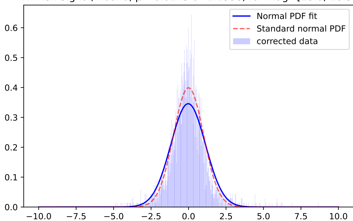
Whiten Signal, y-band, \mu=-0.0242 \sigma=1.0512 ; for mag=[18.0; 18.5]
