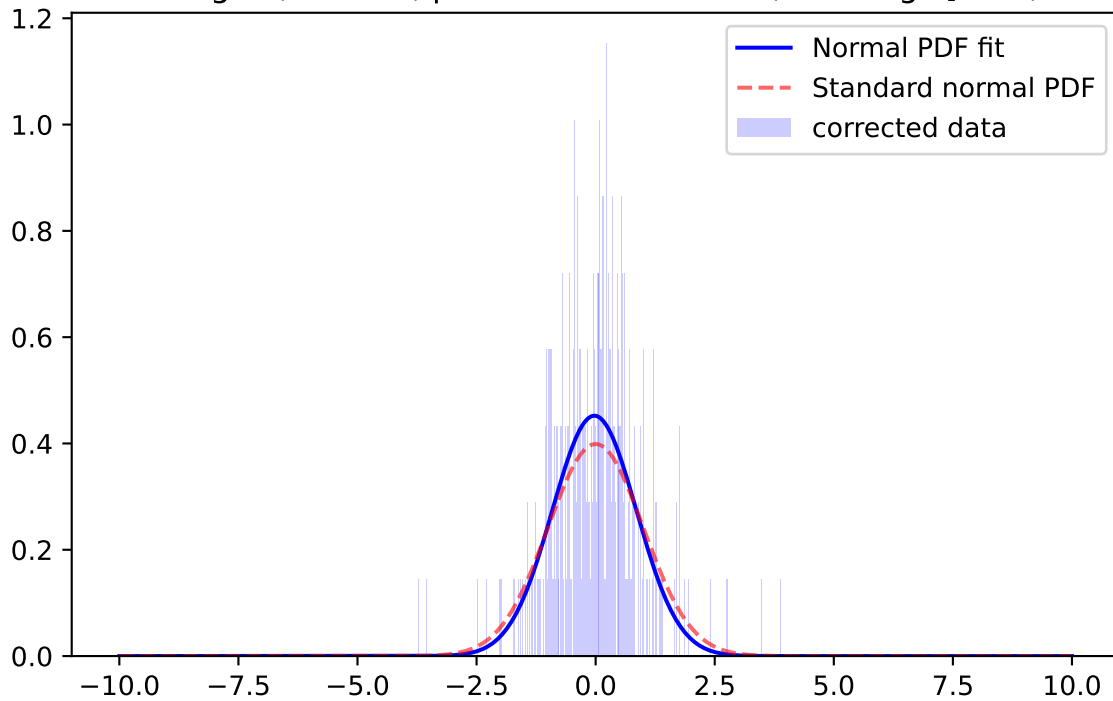
Whiten Signal, r-band, \mu=-0.0305 \sigma=0.9747 ; for mag=[18.0; 18.5]
