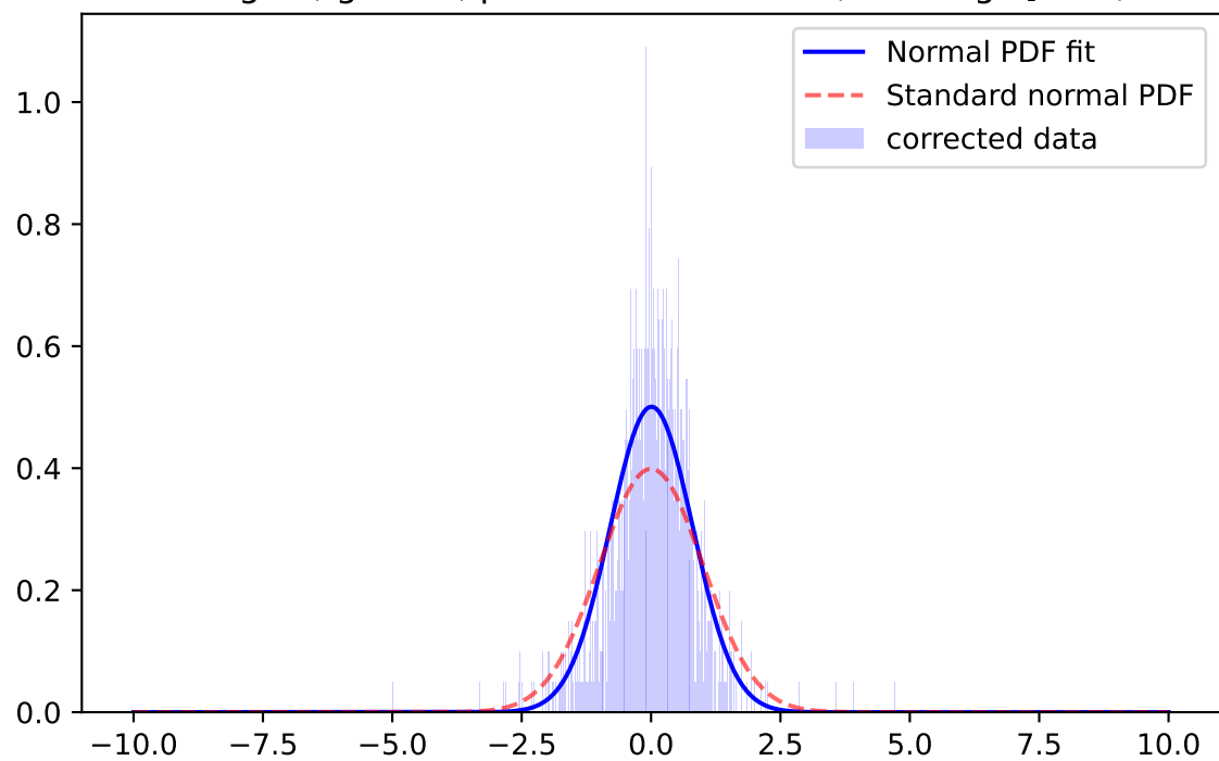
Whiten Signal, i-band, \mu=-0.0245 \sigma=1.1538 ; for mag=[18.0; 18.5]
