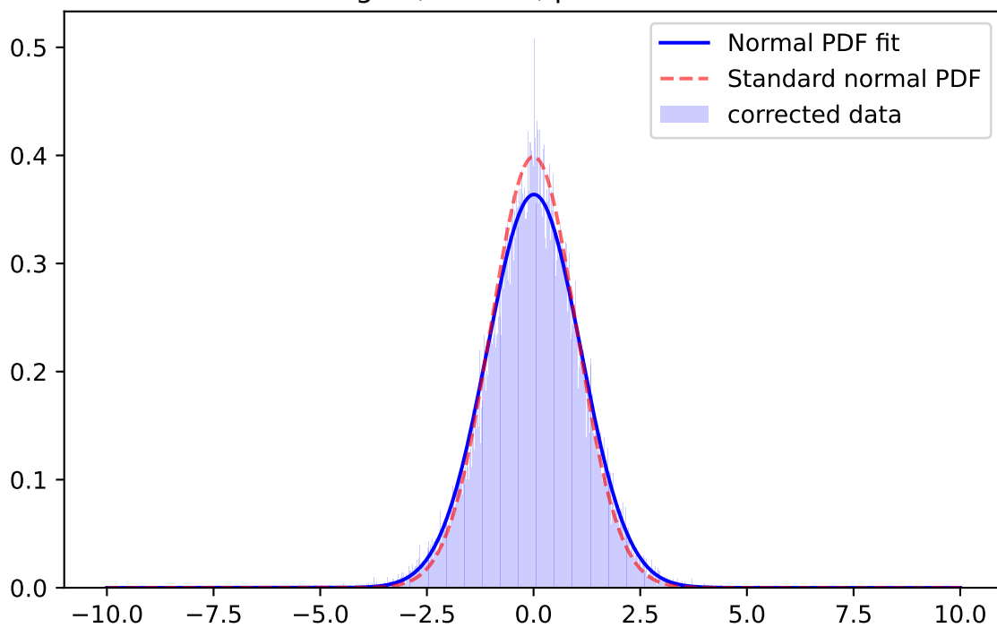
Whiten Signal, r-band, \mu=0.0015 \sigma=1.0063
