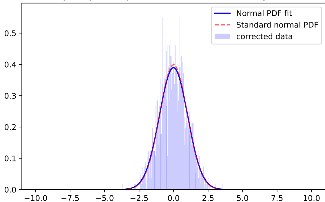
Whiten Signal, i-band, \mu=0.0003 \sigma=1.0259 ; for mag=[21.0; 21.5]
