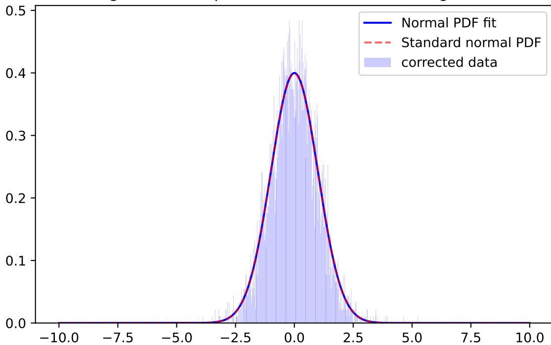
Whiten Signal, z-band, \mu=-0.0082 \sigma=0.9833 ; for mag=[21.0; 21.5]
