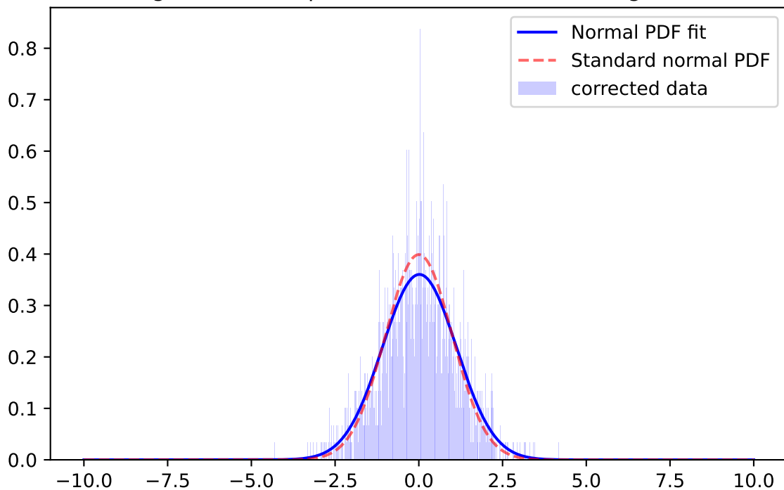
Whiten Signal, r-band, \mu=0.0013 \sigma=0.9977 ; for mag=[21.0; 21.5]
