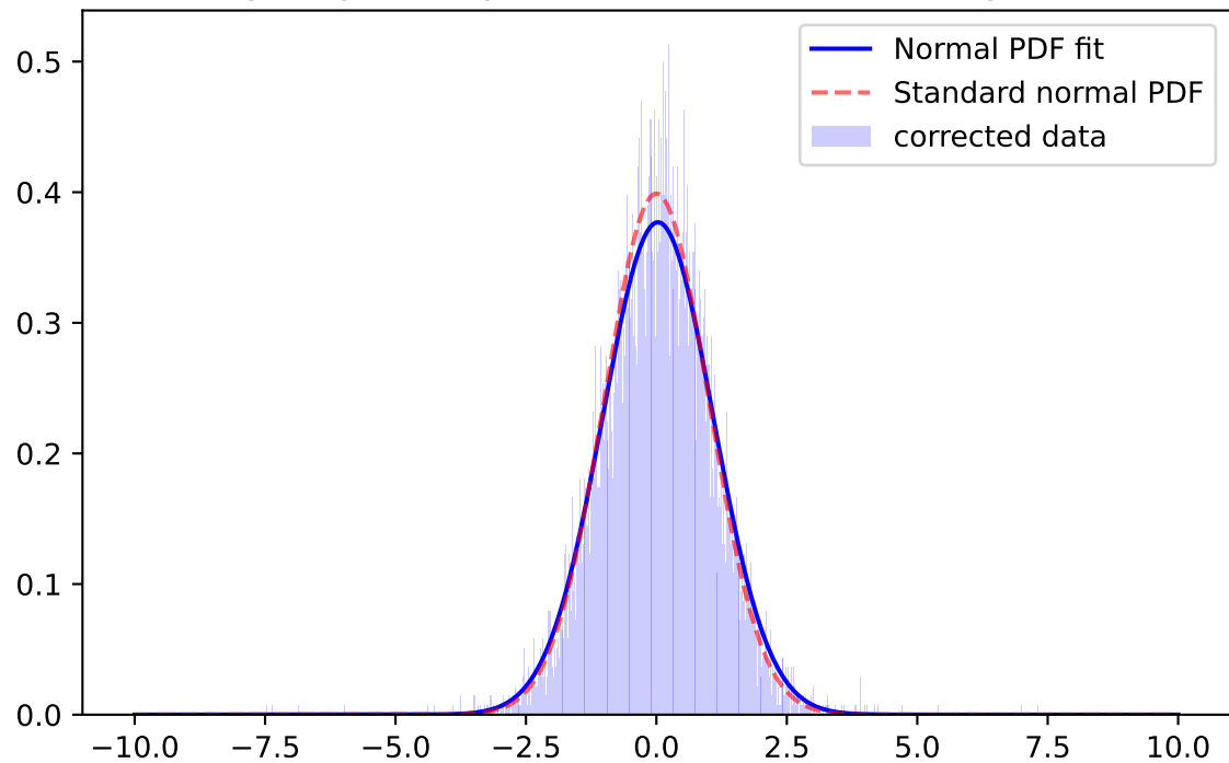
Whiten Signal, y-band, \mu=0.0293 \sigma=1.0583 ; for mag=[21.0; 21.5]
