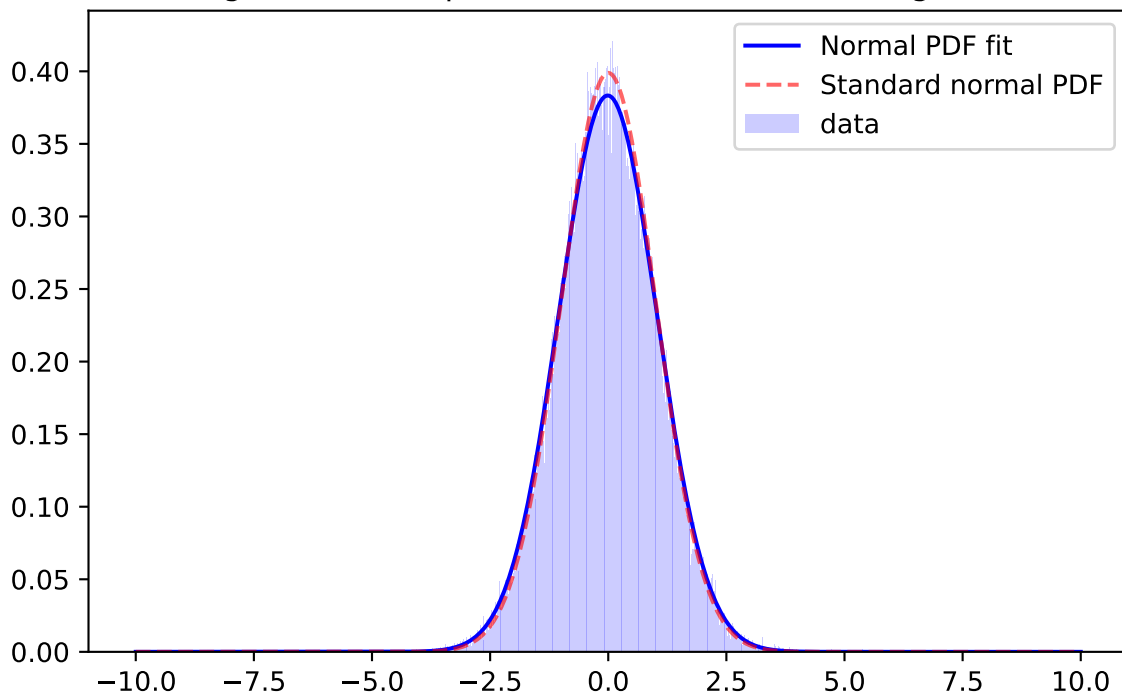
Whiten Signal, r-band, \mu=-0.0208 \sigma=1.0380 ; for mag=[25.0; 25.5]
