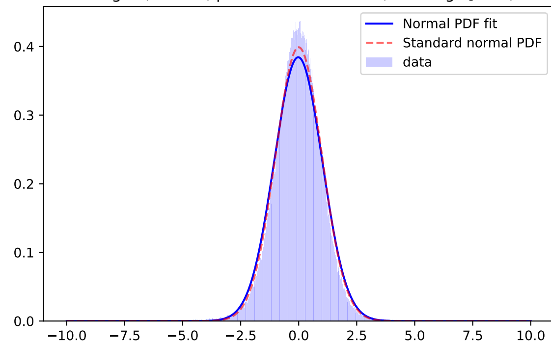
Whiten Signal, z-band, \mu=-0.0378 \sigma=0.9340 ; for mag=[25.0; 25.5]
