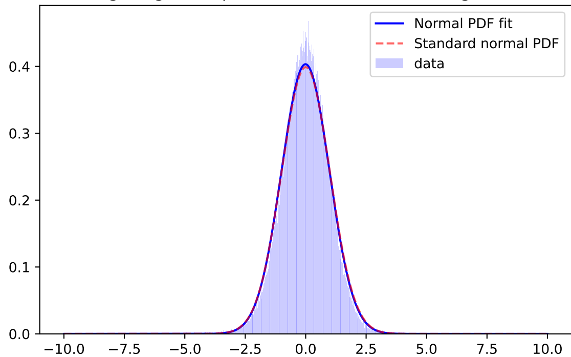
Whiten Signal, i-band, \mu=-0.0096 \sigma=0.9437 ; for mag=[25.0; 25.5]
