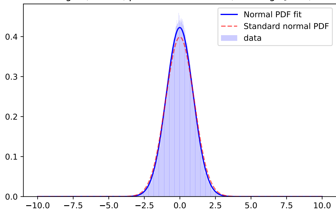
Whiten Signal, y-band, \mu=-0.0336 \sigma=0.9572 ; for mag=[25.0; 25.5]
