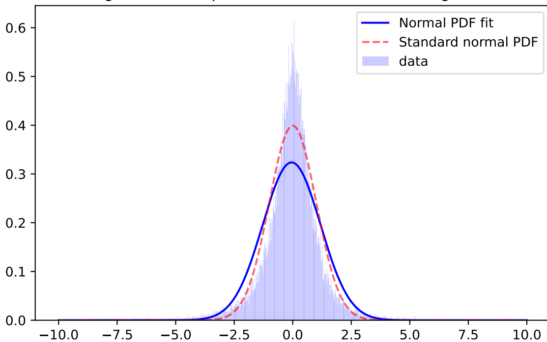
Whiten Signal, z-band, \mu=-0.0487 \sigma=1.2323 ; for mag=[18.0; 18.5]
