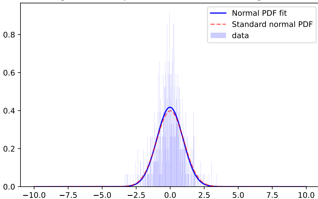
Whiten Signal, r-band, \mu=0.0764 \sigma=1.1658 ; for mag=[18.0; 18.5]
