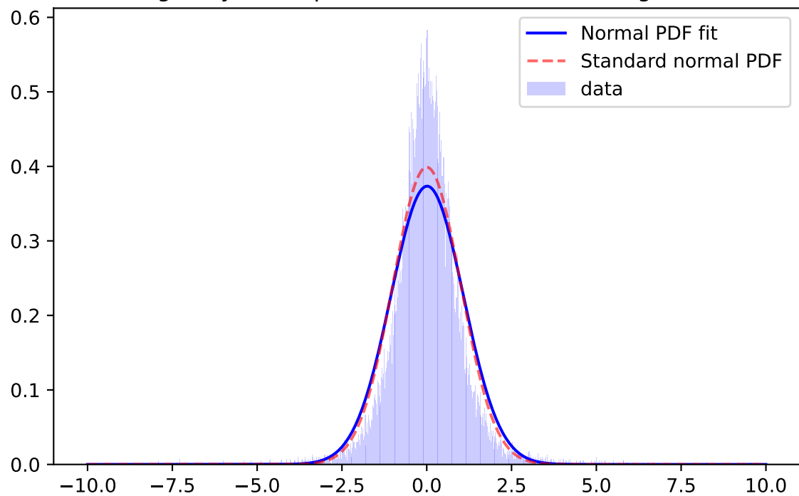
Whiten Signal, y-band, \mu=0.0126 \sigma=1.0683 ; for mag=[18.0; 18.5]
