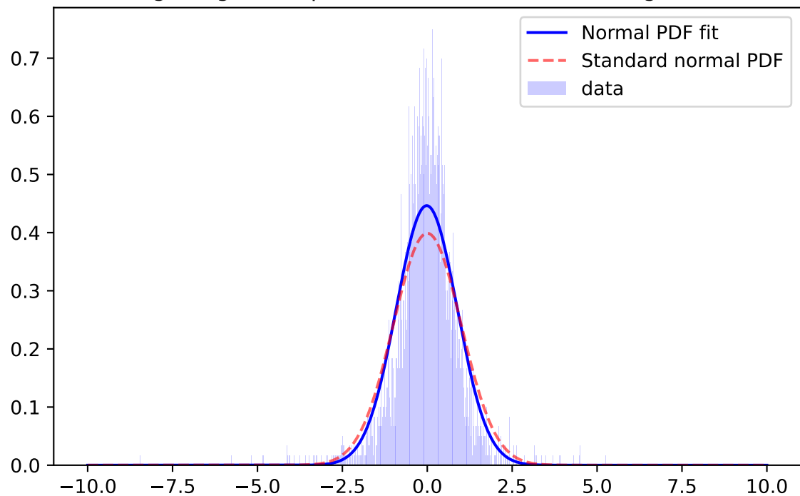
Whiten Signal, i-band, \mu=0.0704 \sigma=1.2247 ; for mag=[18.0; 18.5]
