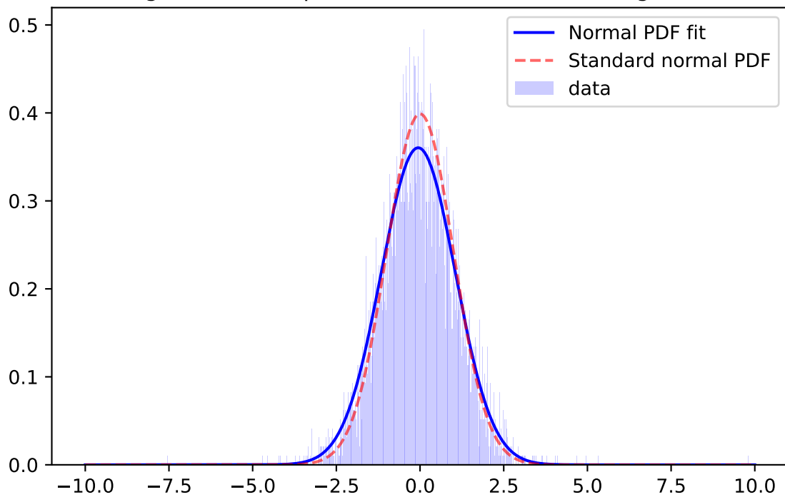
Whiten Signal, r-band, \mu=0.0274 \sigma=1.3789 ; for mag=[21.0; 21.5]
