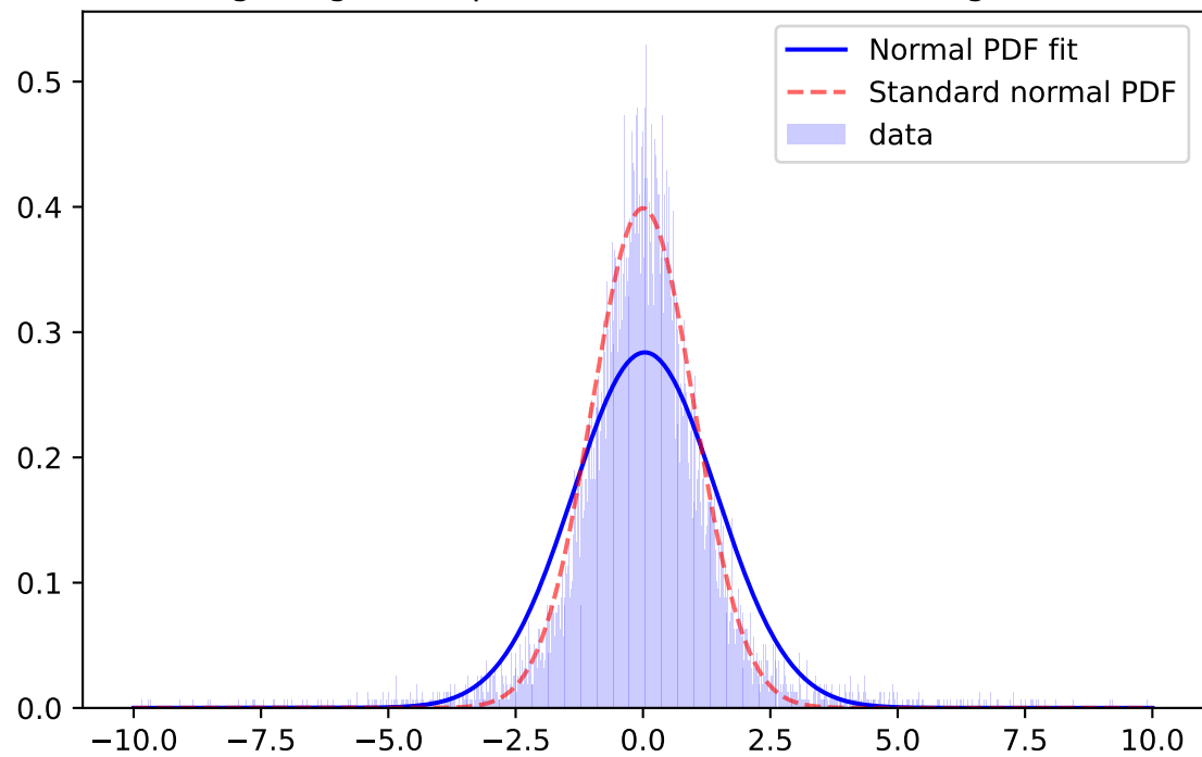
Whiten Signal, i-band, \mu=-0.0313 \sigma=1.3444 ; for mag=[21.0; 21.5]
