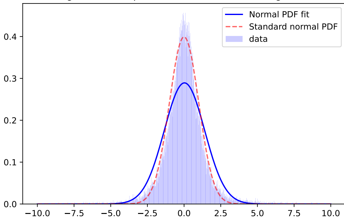
Whiten Signal, z-band, \mu=-0.1424 \sigma=1.1865 ; for mag=[21.0; 21.5]
