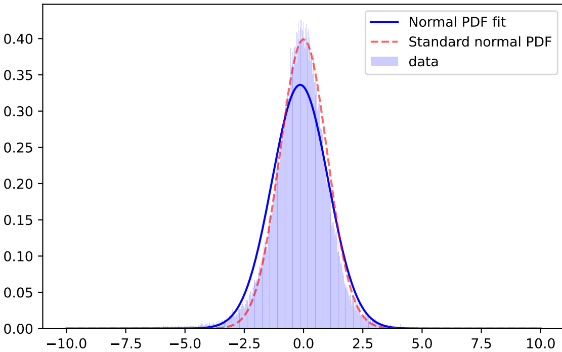
Whiten Signal, z-band, \mu=-0.1424 \sigma=1.1865 ; for mag=[21.0; 21.5]
