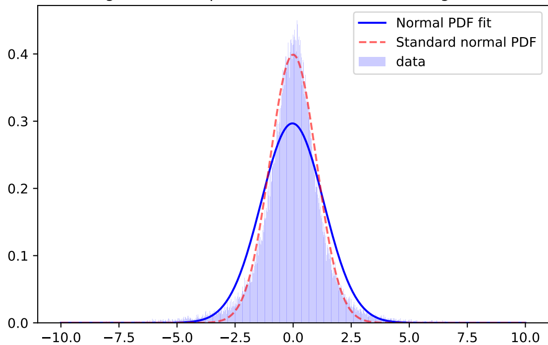
Whiten Signal, y-band, \mu=0.0054 \sigma=1.1945 ; for mag=[21.0; 21.5]
