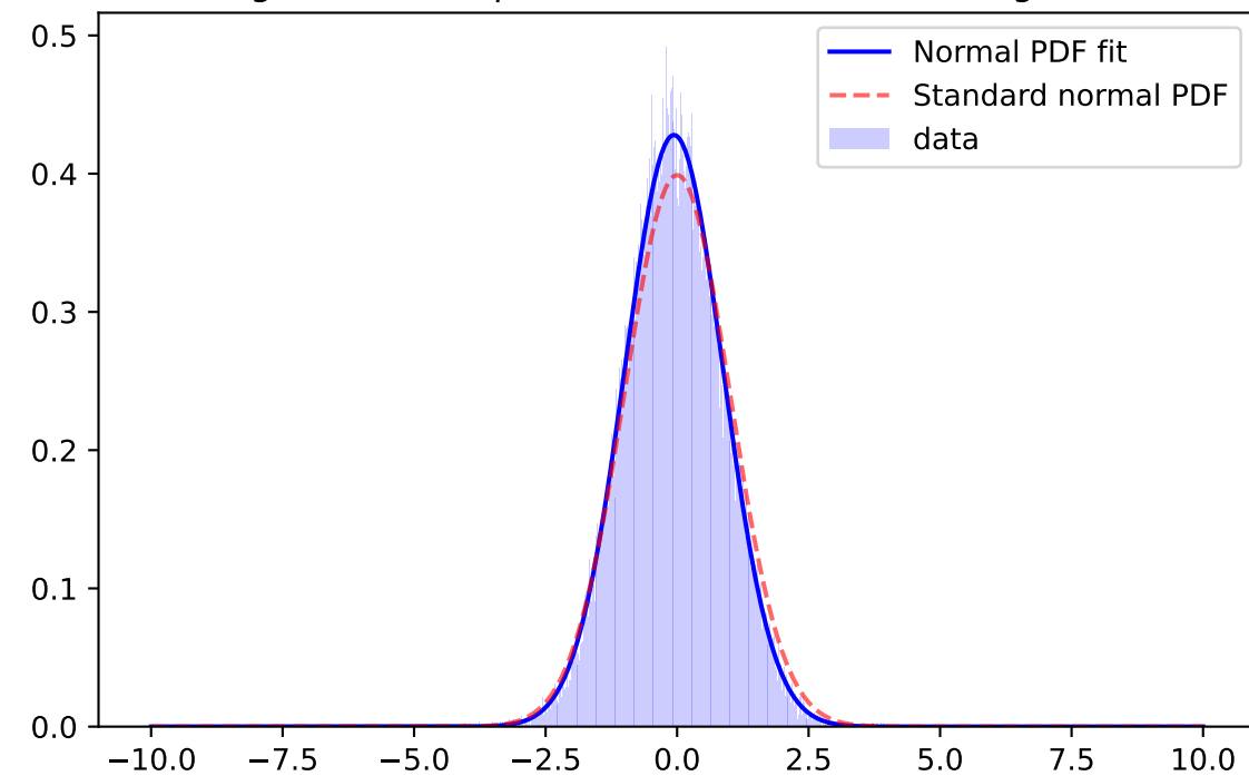
Whiten Signal, z-band, \mu=-0.0603 \sigma=0.9321 ; for mag=[25.0; 25.5]
