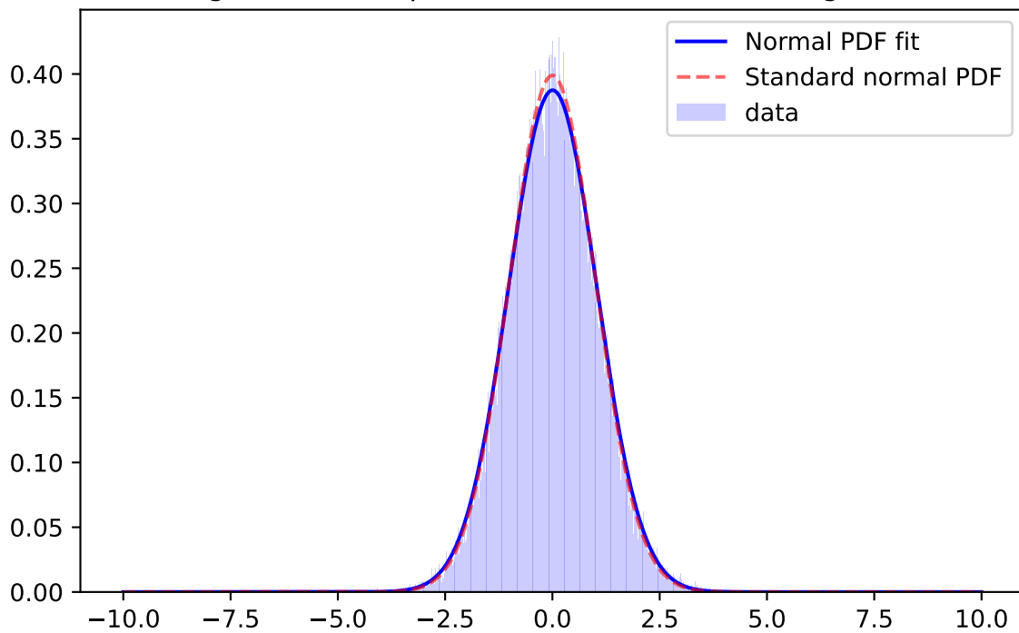
Whiten Signal, r-band, \mu=-0.0147 \sigma=1.0102 ; for mag=[25.0; 25.5]
