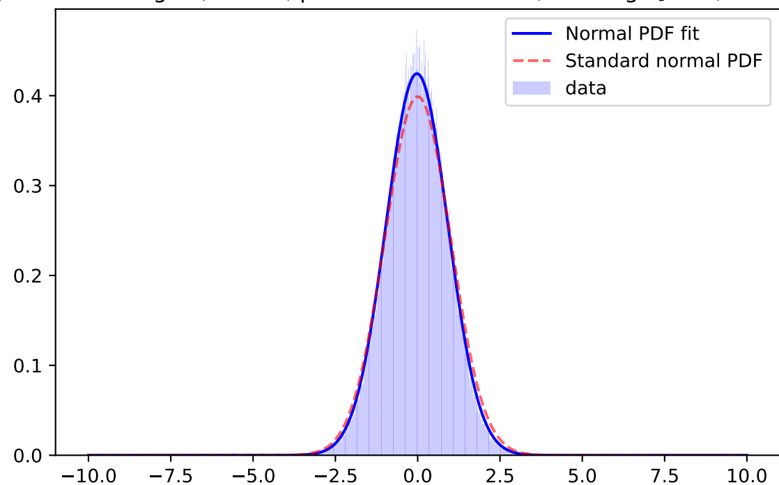
Whiten Signal, y-band, \mu=-0.0611 \sigma=0.9396 ; for mag=[25.0; 25.5]
