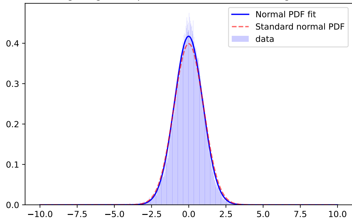
Whiten Signal, i-band, \mu=-0.0226 \sigma=0.9397 ; for mag=[25.0; 25.5]
