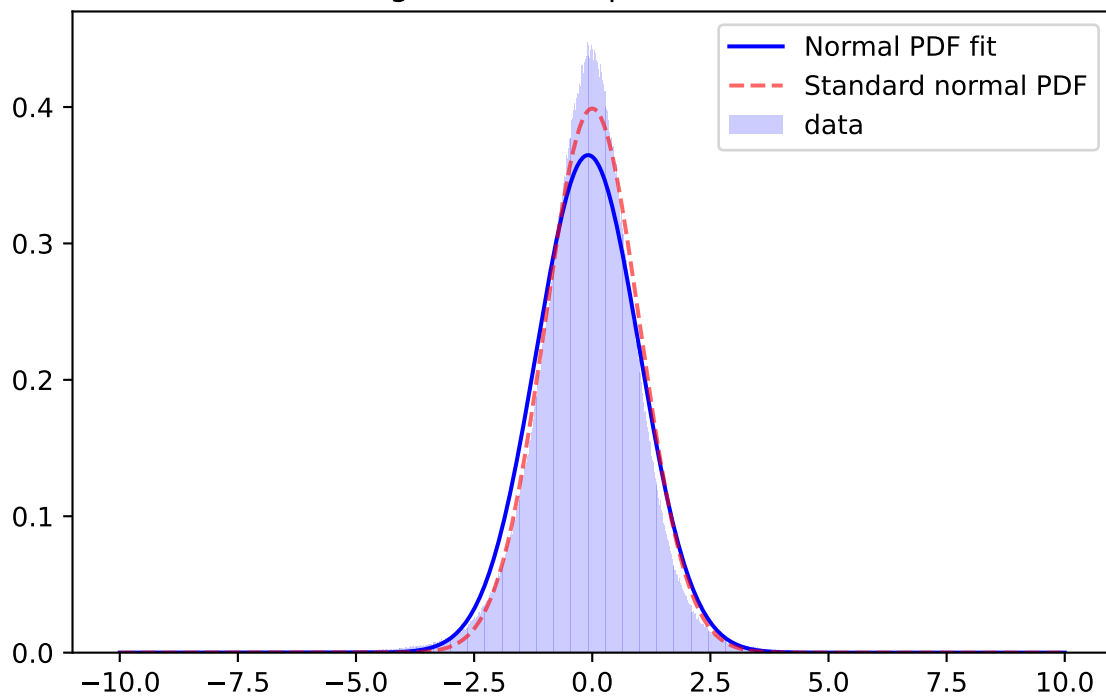
Whiten Signal, z-band, \mu=-0.0874 \sigma=1.0937
