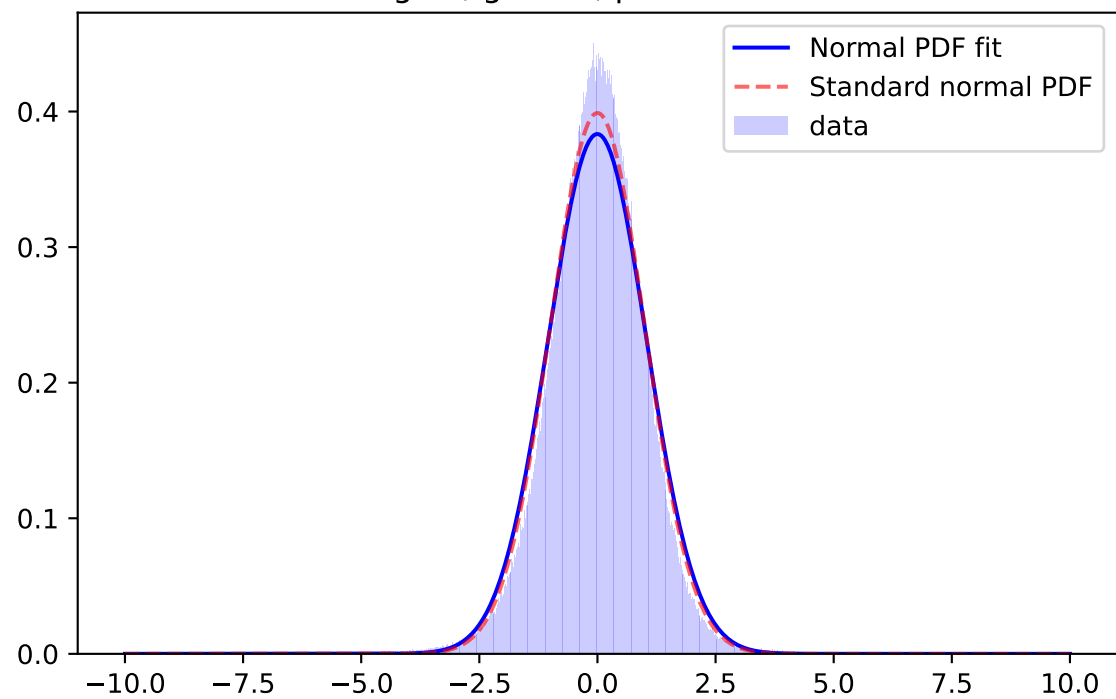
Whiten Signal, i-band, \mu=-0.0363 \sigma=1.1330
