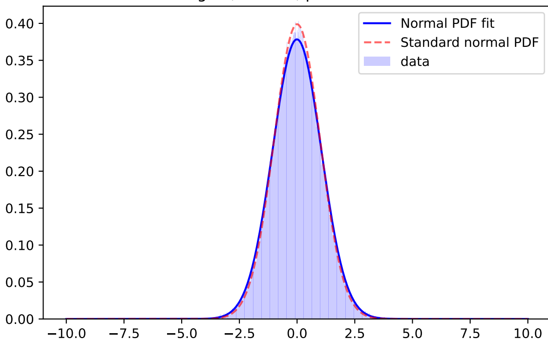
Whiten Signal, r-band, \mu=-0.0102 \sigma=1.1234
