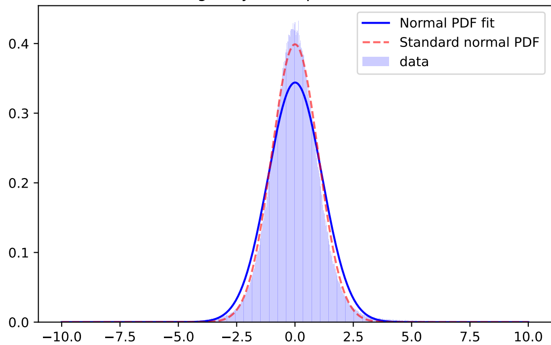
Whiten Signal, y-band, \mu=0.0061 \sigma=1.1596
