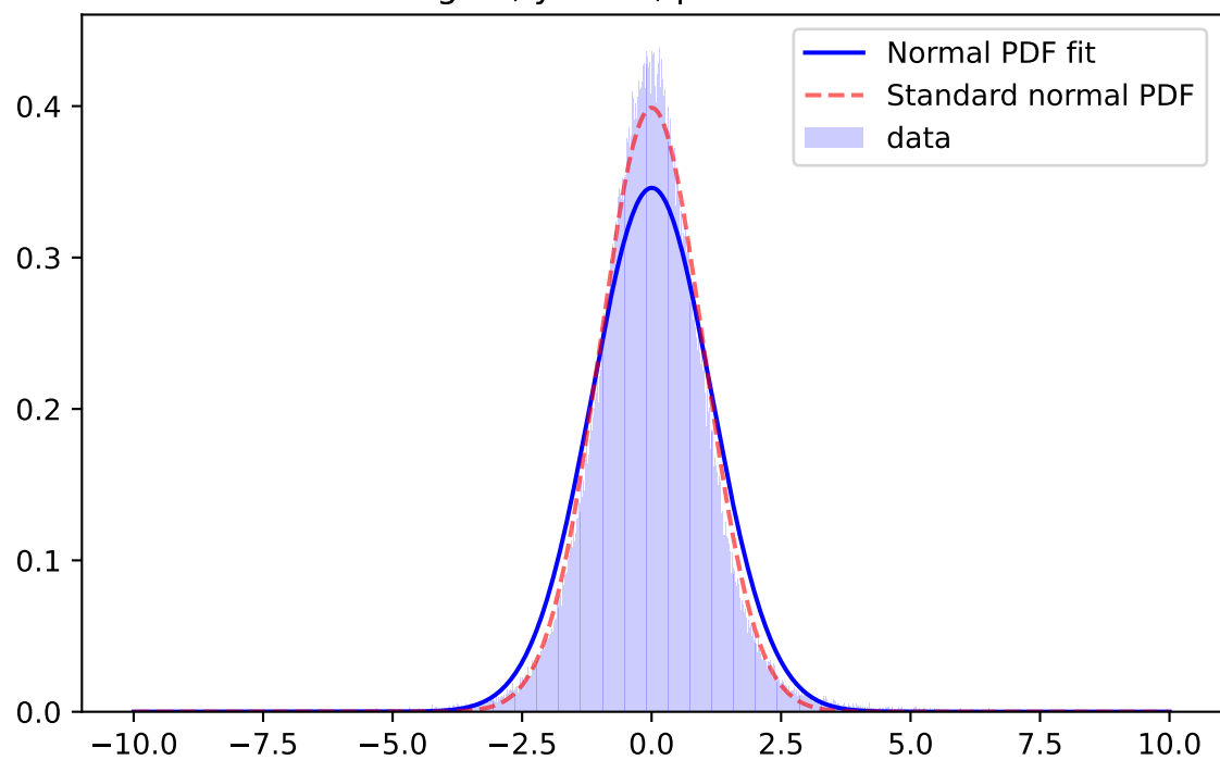
Whiten Signal, y-band, \mu=0.0039 \sigma=1.1530
