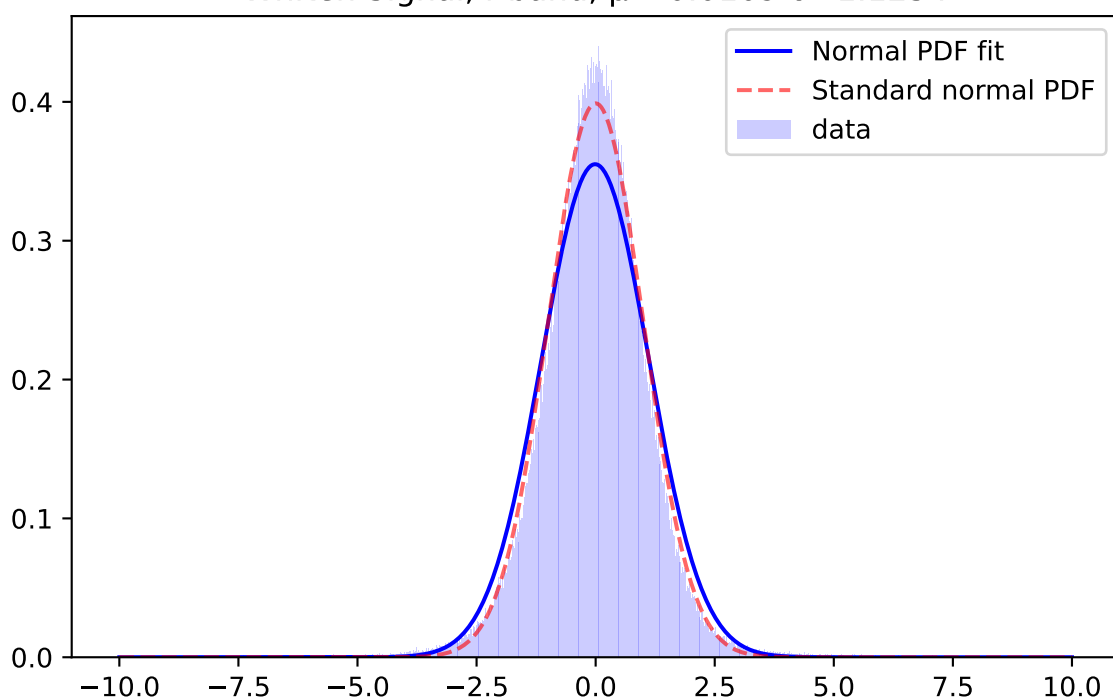
Whiten Signal, z-band, \mu=-0.0834 \sigma=1.0908
