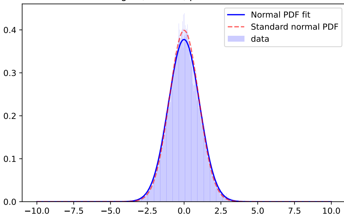
Whiten Signal, r-band, \mu=-0.0109 \sigma=1.1234
