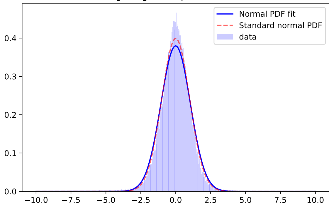
Whiten Signal, i-band, \mu=-0.0398 \sigma=1.1433
