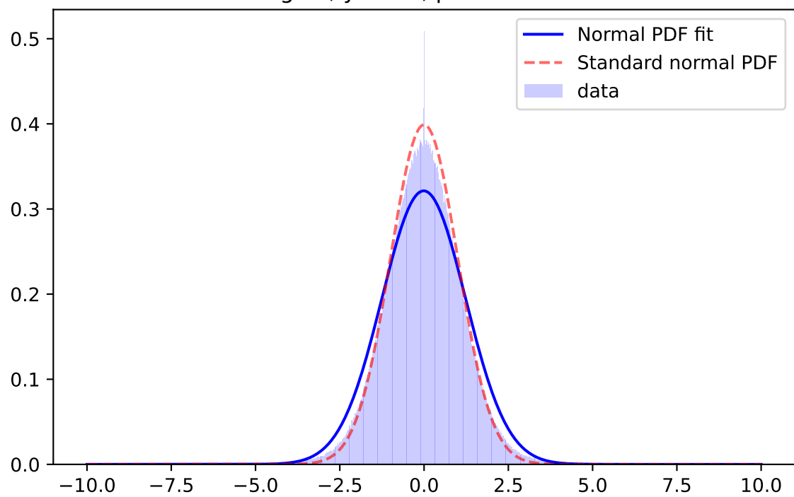
Whiten Signal, y-band, \mu=-0.0104 \sigma=1.2415
