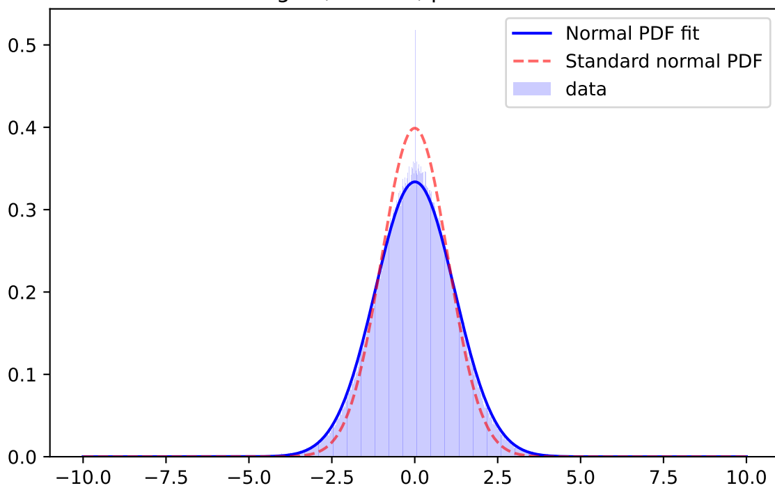
Whiten Signal, r-band, \mu=-0.0040 \sigma=1.2092
