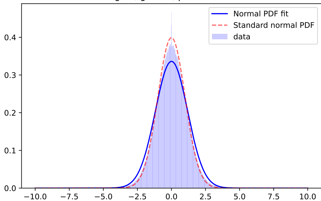
Whiten Signal, i-band, \mu=-0.0170 \sigma=1.2553
