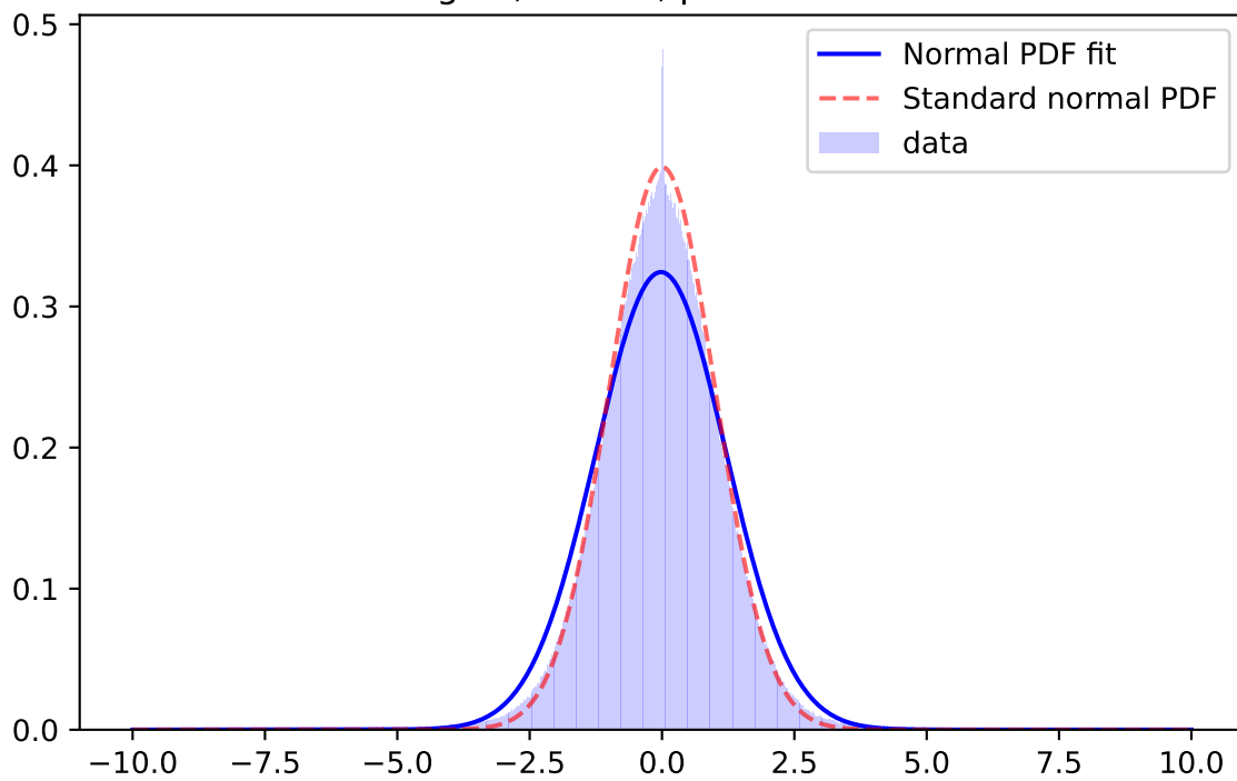
Whiten Signal, z-band, \mu=-0.0201 \sigma=1.2299
