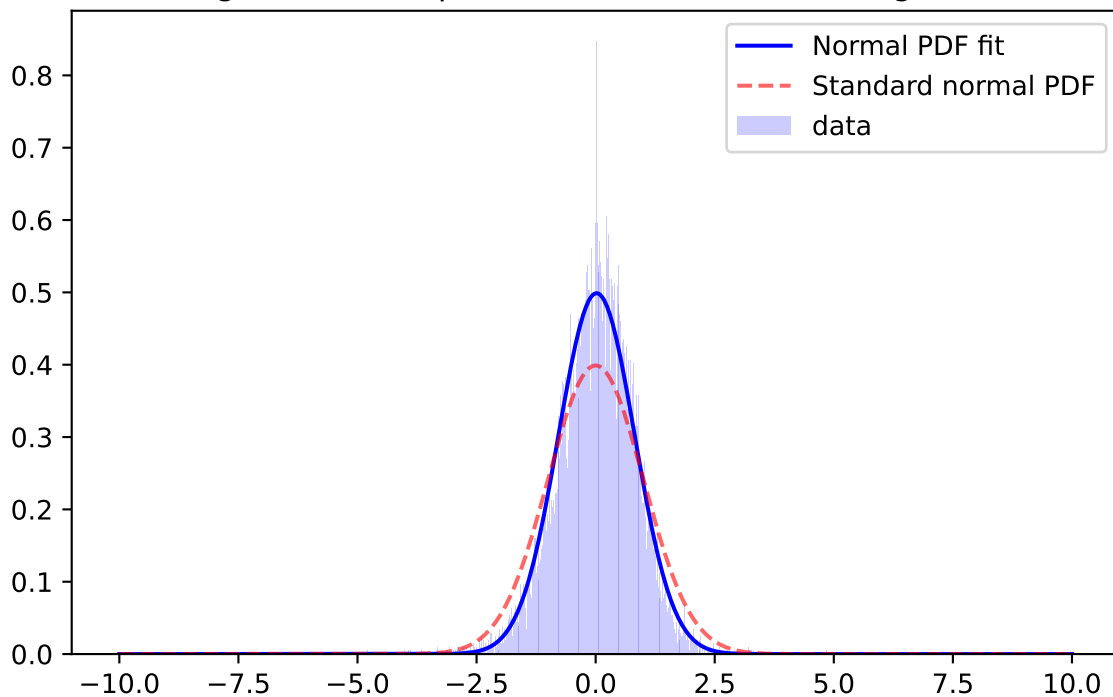
Whiten Signal, r-band, \mu=0.0132 \sigma=0.9902 ; for mag=[21.0; 21.5]
