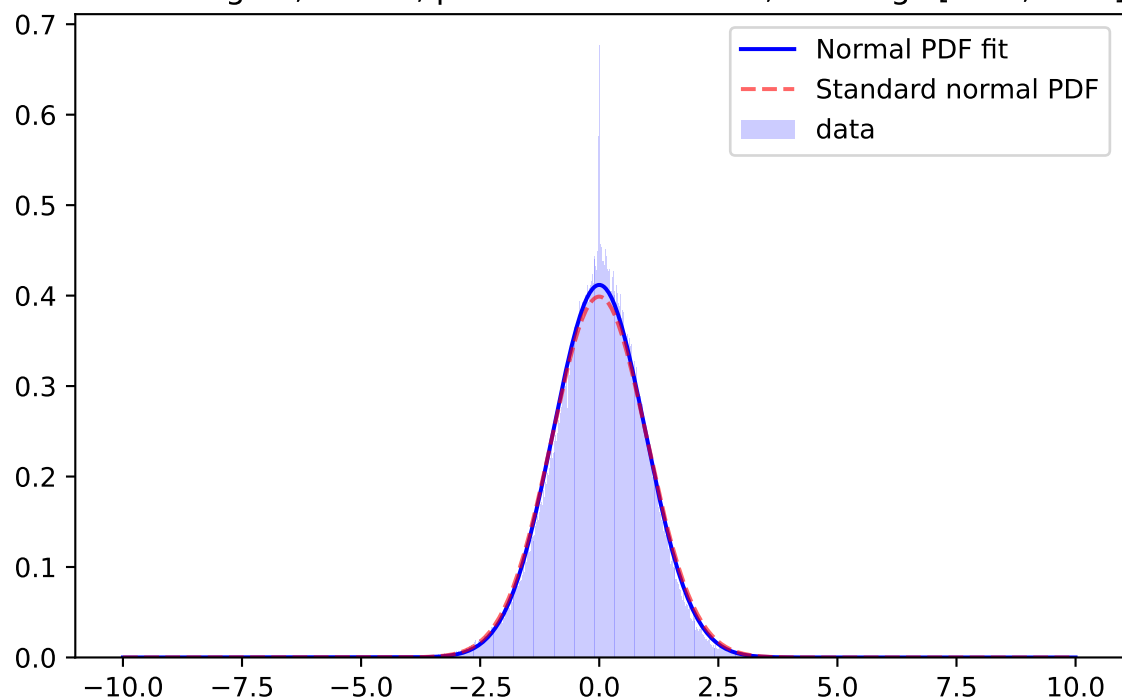
Whiten Signal, y-band, \mu=0.0292 \sigma=1.0586 ; for mag=[21.0; 21.5]
