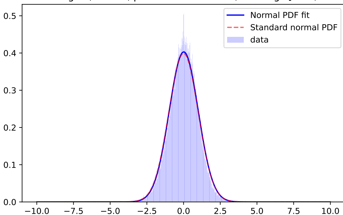
Whiten Signal, z-band, \mu=0.0074 \sigma=0.9837 ; for mag=[21.0; 21.5]
