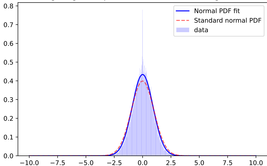
Whiten Signal, i-band, \mu=0.0003 \sigma=0.9686 ; for mag=[21.0; 21.5]
