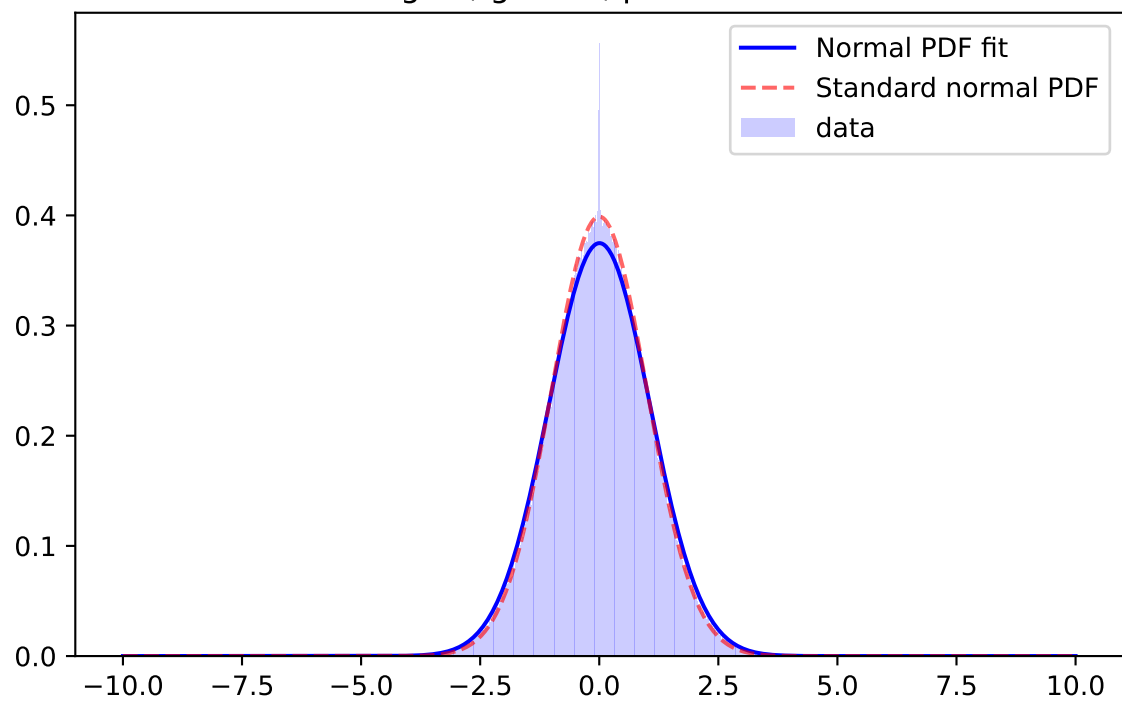
Whiten Signal, i-band, \mu=0.0027 \sigma=1.0759
