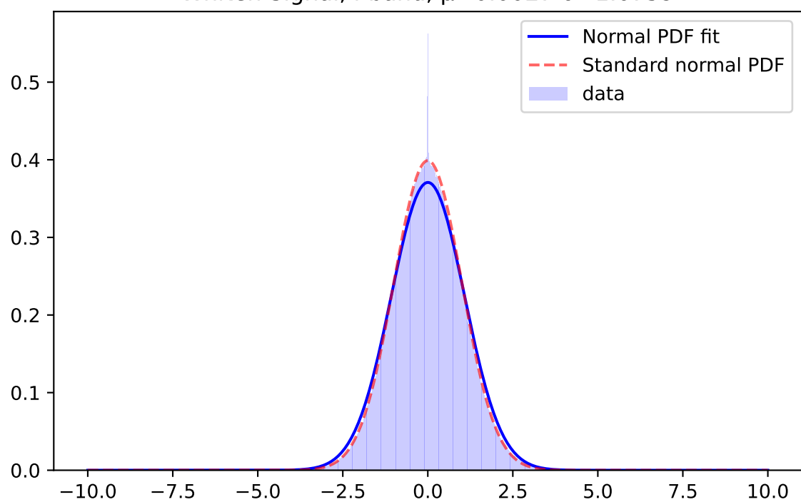
Whiten Signal, y-band, \mu=0.0139 \sigma=1.0419
