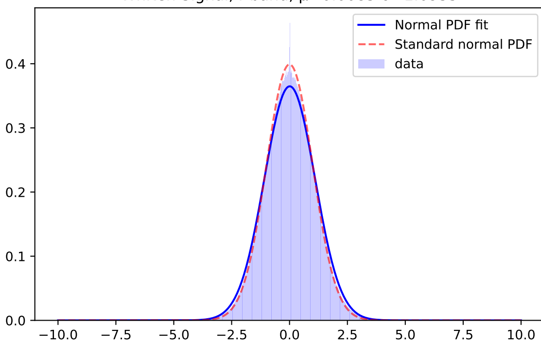
Whiten Signal, z-band, \mu=0.0069 \sigma=1.0499
