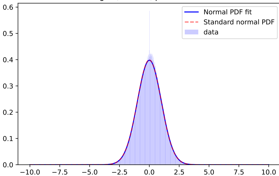
Whiten Signal, r-band, \mu=0.0085 \sigma=1.0935
