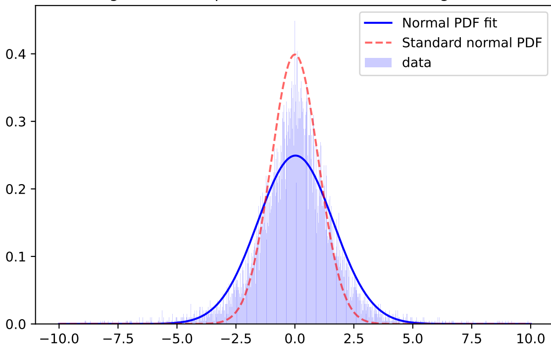
Whiten Signal, z-band, \mu=-0.0117 \sigma=1.2236 ; for mag=[18.0; 18.5]
