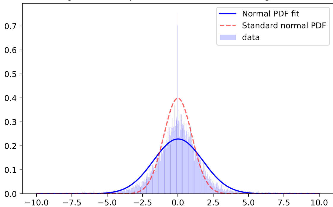
Whiten Signal, y-band, \mu=0.0368 \sigma=0.9622 ; for mag=[18.0; 18.5]
