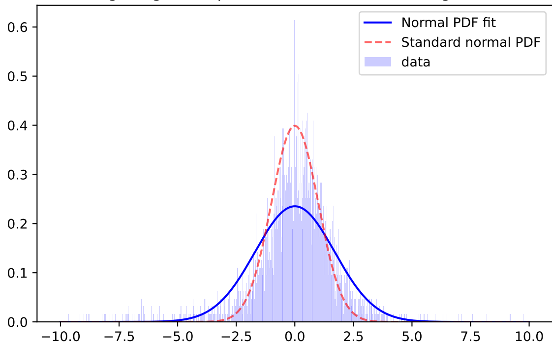
Whiten Signal, i-band, \mu=0.0189 \sigma=1.7440 ; for mag=[18.0; 18.5]
