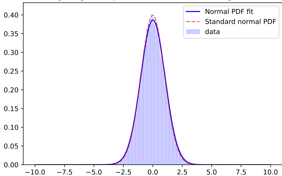
Whiten Signal, i-band, \mu=0.0028 \sigma=0.9982 ; for mag=[25.0; 25.5]
