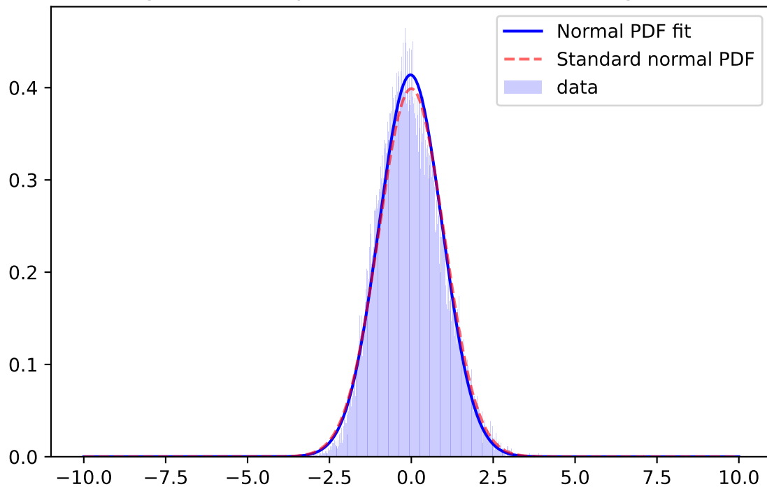
Whiten Signal, z-band, \mu=-0.0230 \sigma=0.9639 ; for mag=[25.0; 25.5]
