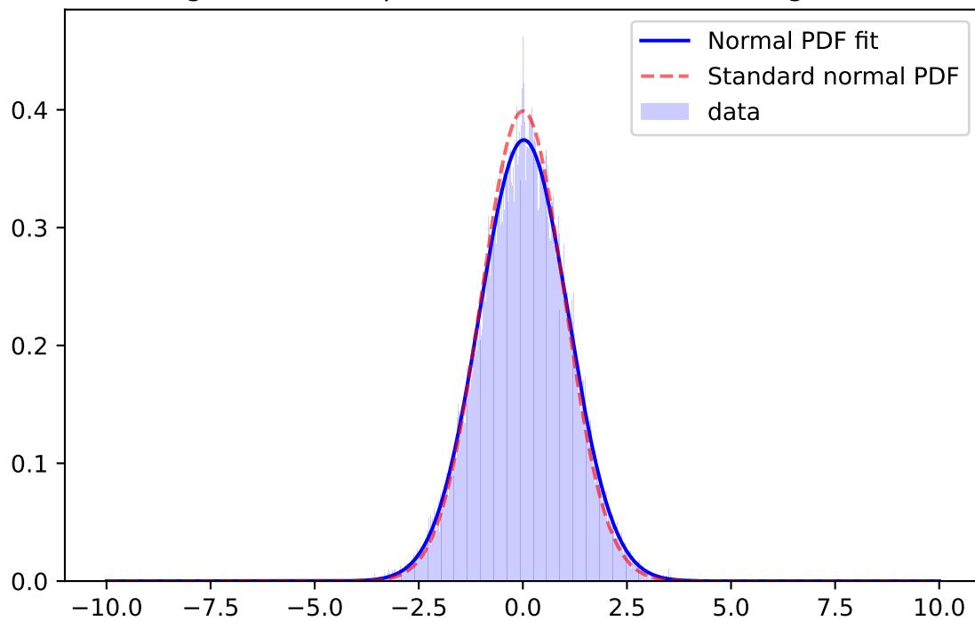
Whiten Signal, r-band, \mu=0.0022 \sigma=1.0417 ; for mag=[25.0; 25.5]
