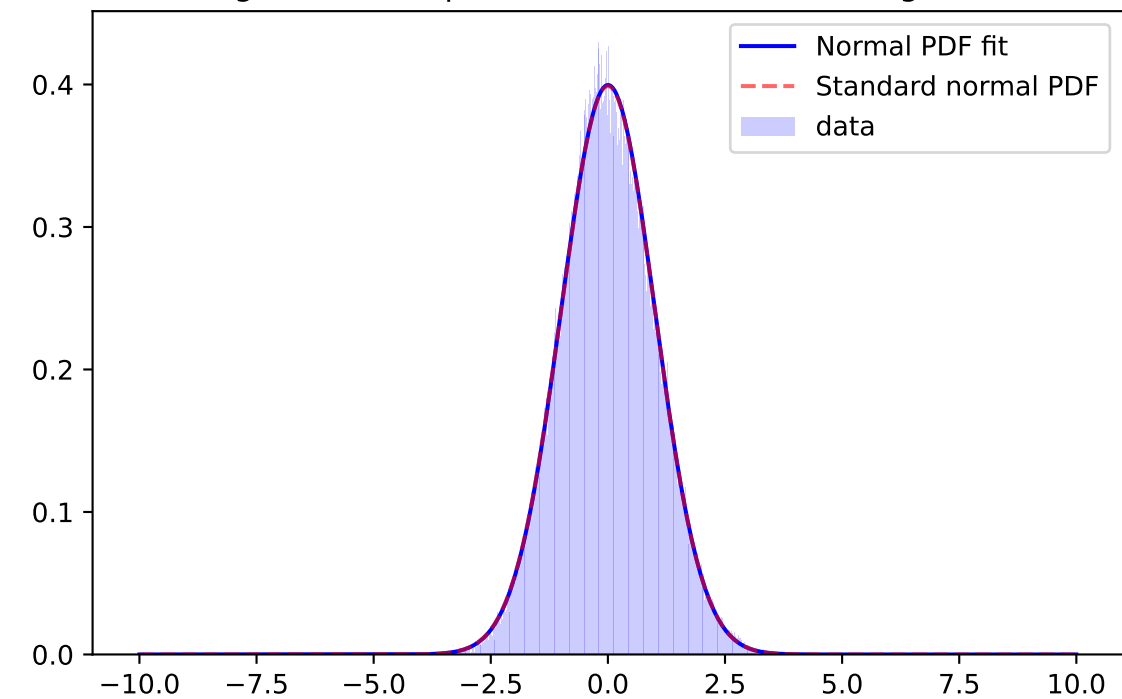
Whiten Signal, y-band, \mu=-0.0629 \sigma=0.8806 ; for mag=[25.0; 25.5]
