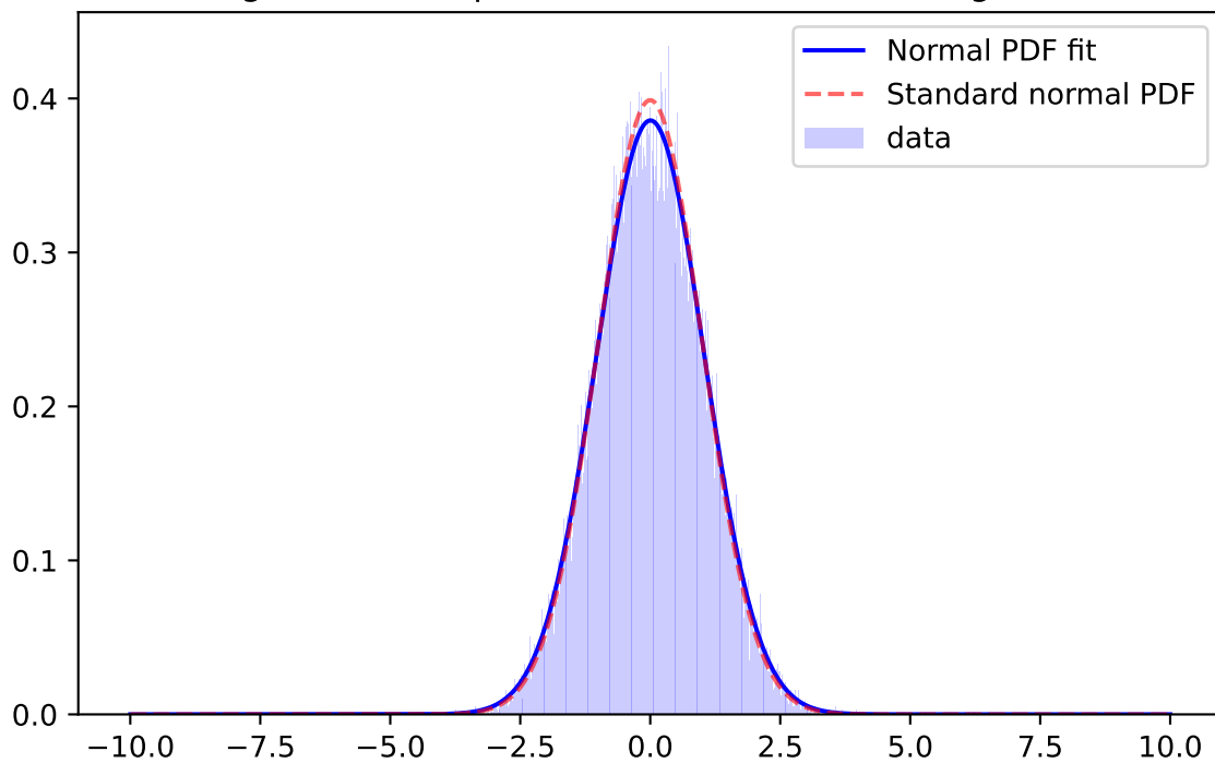
Whiten Signal, z-band, \mu=-0.0282 \sigma=0.9553 ; for mag=[25.0; 25.5]
