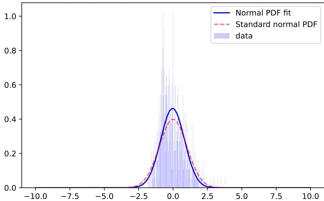
Whiten Signal, y-band, \mu=-0.0322 \sigma=0.8639 ; for mag=[25.0; 25.5]
