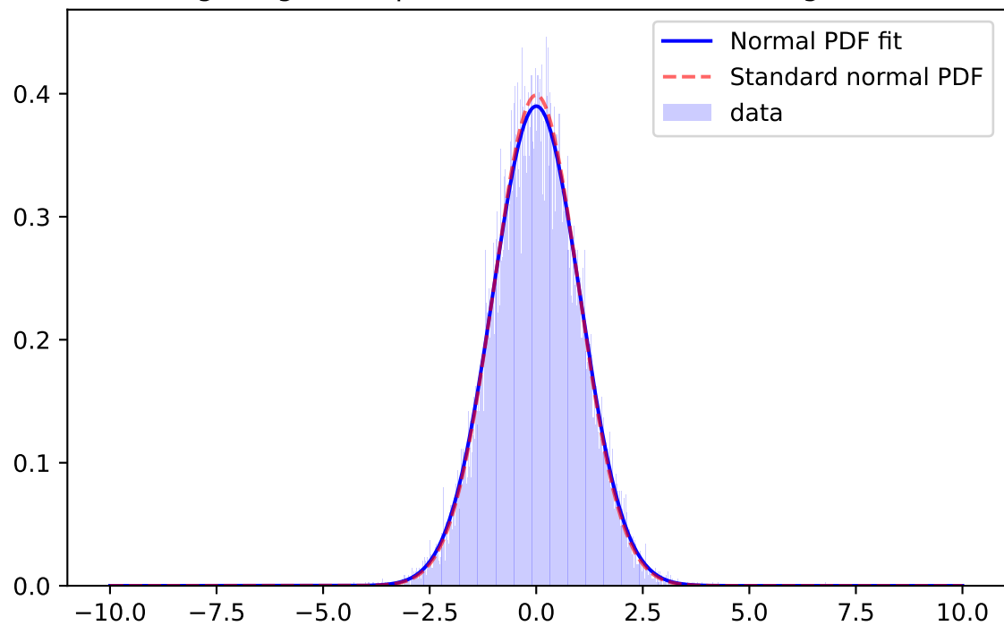
Whiten Signal, i-band, \mu=-0.0068 \sigma=1.0006 ; for mag=[25.0; 25.5]
