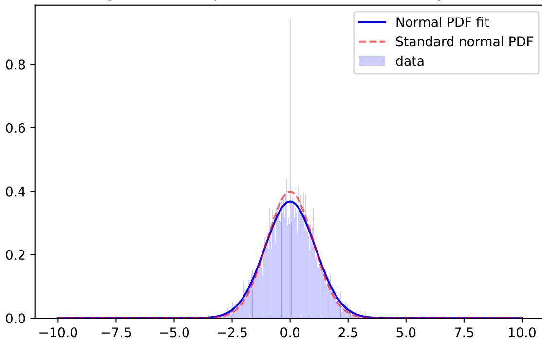
Whiten Signal, r-band, \mu=0.0040 \sigma=1.0341 ; for mag=[25.0; 25.5]
