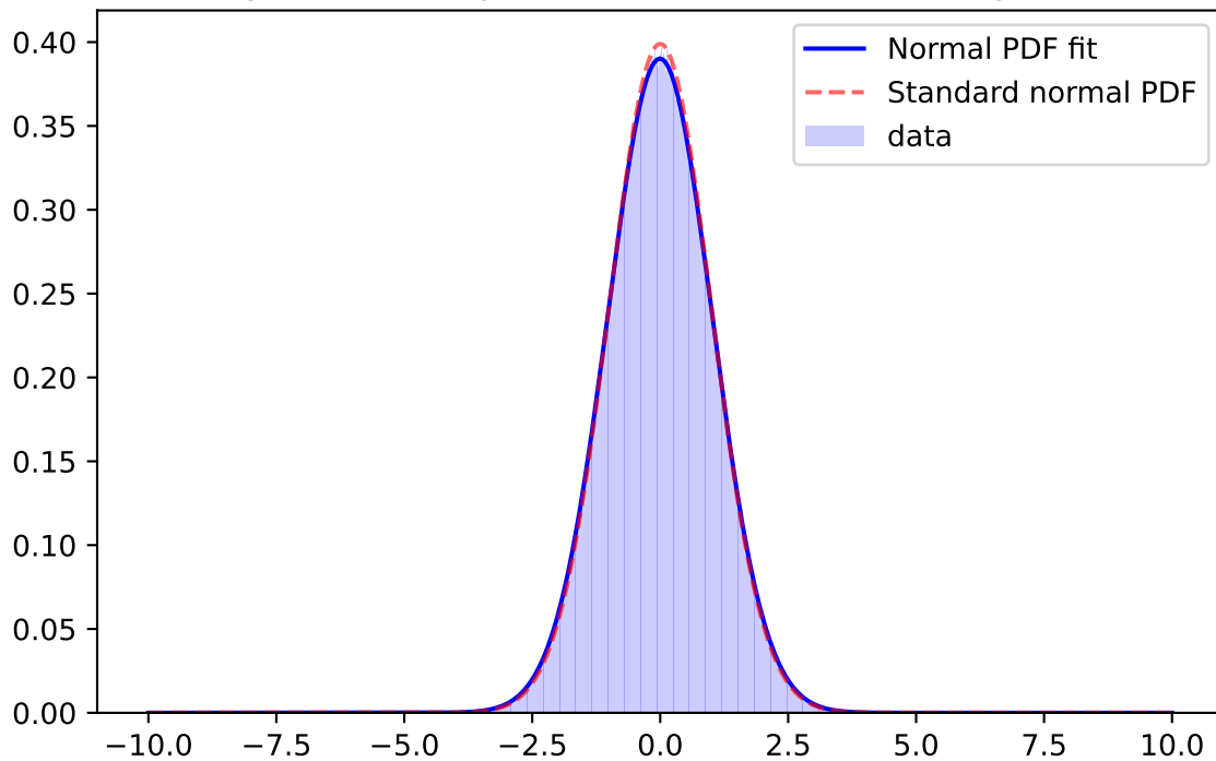
Whiten Signal, z-band, \mu=-0.0057 \sigma=1.0226 ; for mag=[25.0; 25.5]
