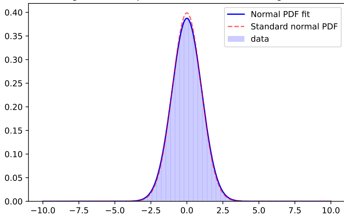
Whiten Signal, y-band, \mu=-0.0131 \sigma=1.0197 ; for mag=[25.0; 25.5]
