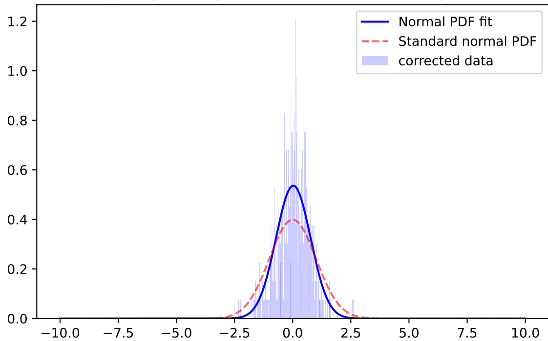
Whiten Signal, y-band, \mu=0.0259 \sigma=0.7438 ; for mag=[18.0; 18.5]
