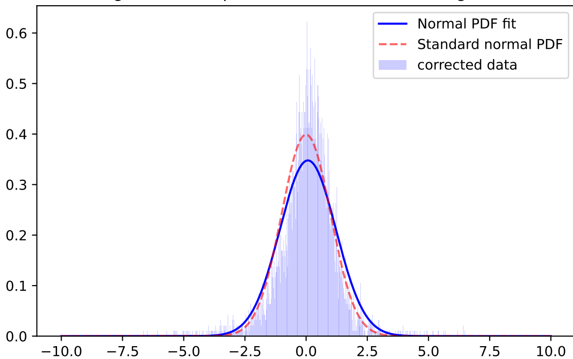
Whiten Signal, z-band, \mu=0.0607 \sigma=1.0089 ; for mag=[18.0; 18.5]
