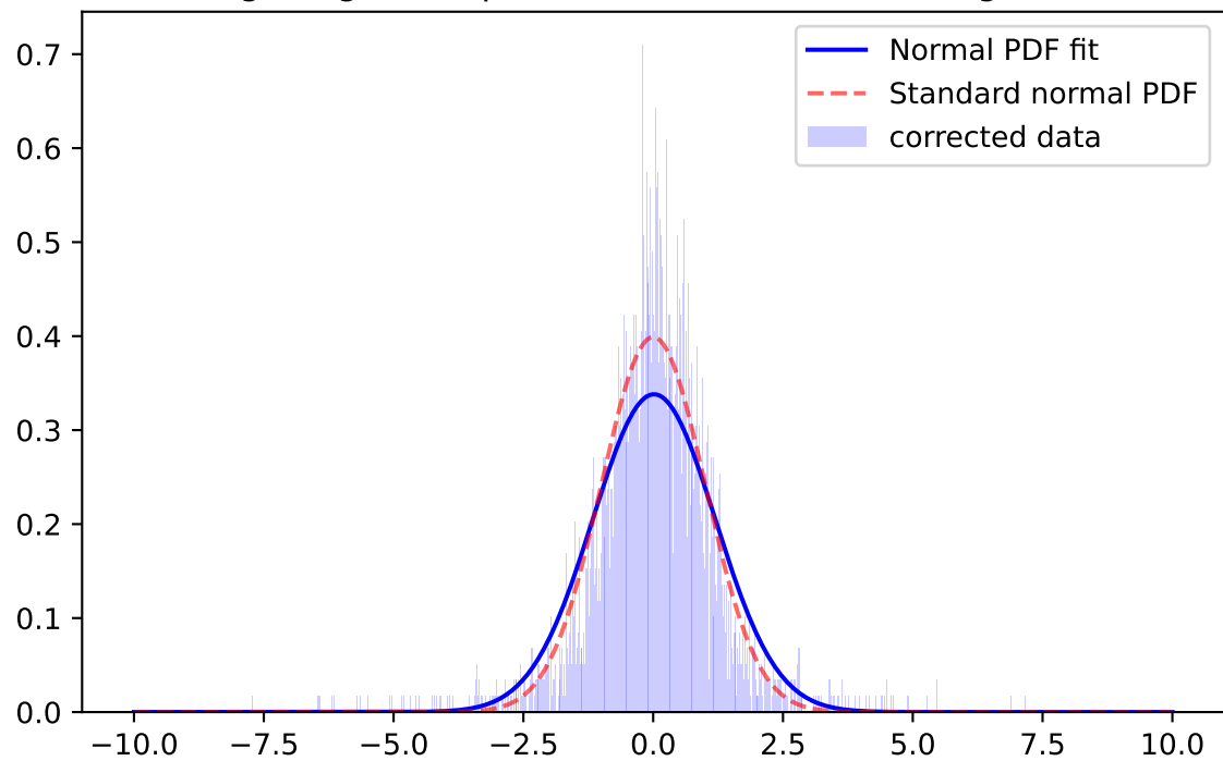
Whiten Signal, i-band, \mu=0.0424 \sigma=1.3336 ; for mag=[18.0; 18.5]
