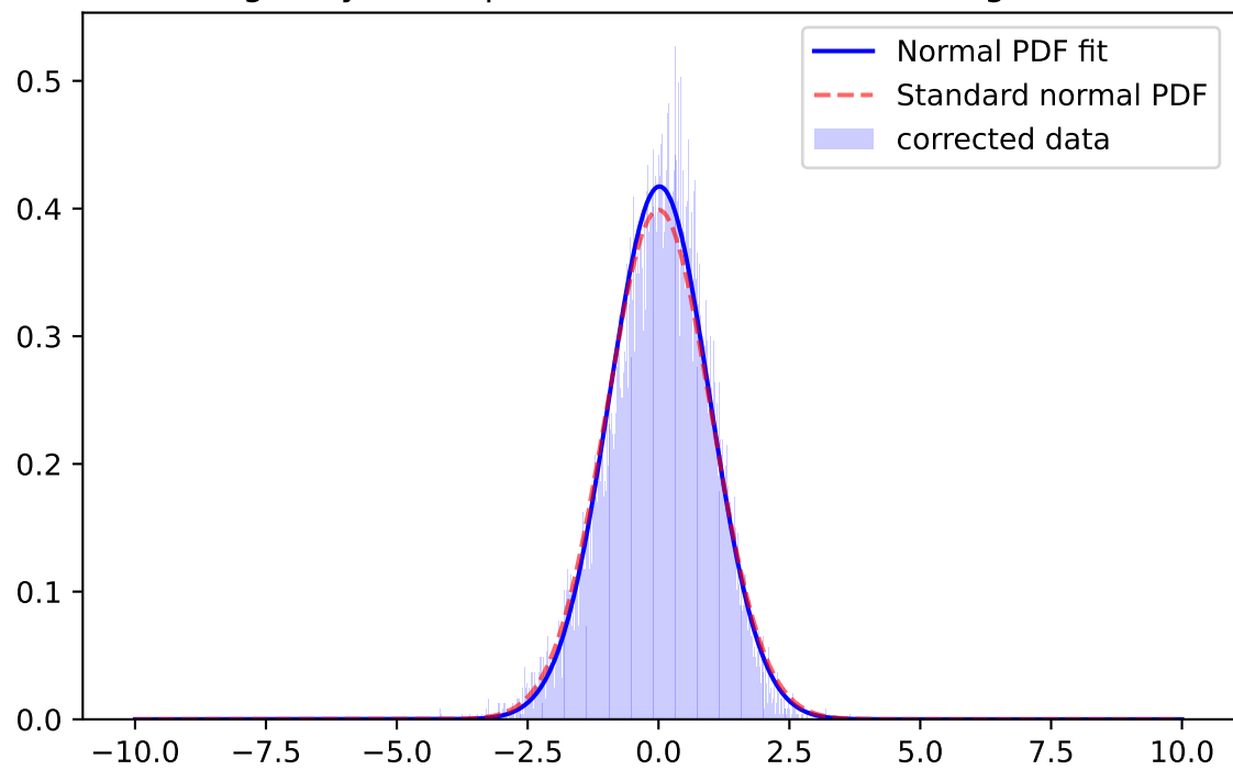
Whiten Signal, y-band, \mu=0.0182 \sigma=0.9559 ; for mag=[21.0; 21.5]
