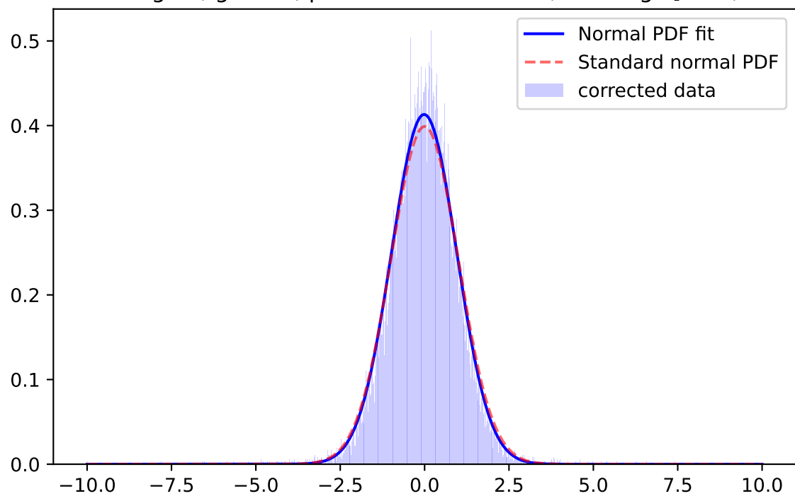
Whiten Signal, i-band, \mu=0.0063 \sigma=0.9299 ; for mag=[21.0; 21.5]
