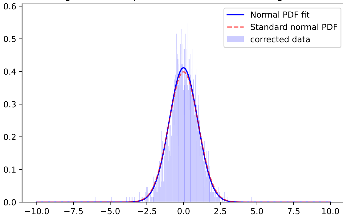
Whiten Signal, r-band, \mu=0.0069 \sigma=0.9615 ; for mag=[21.0; 21.5]
