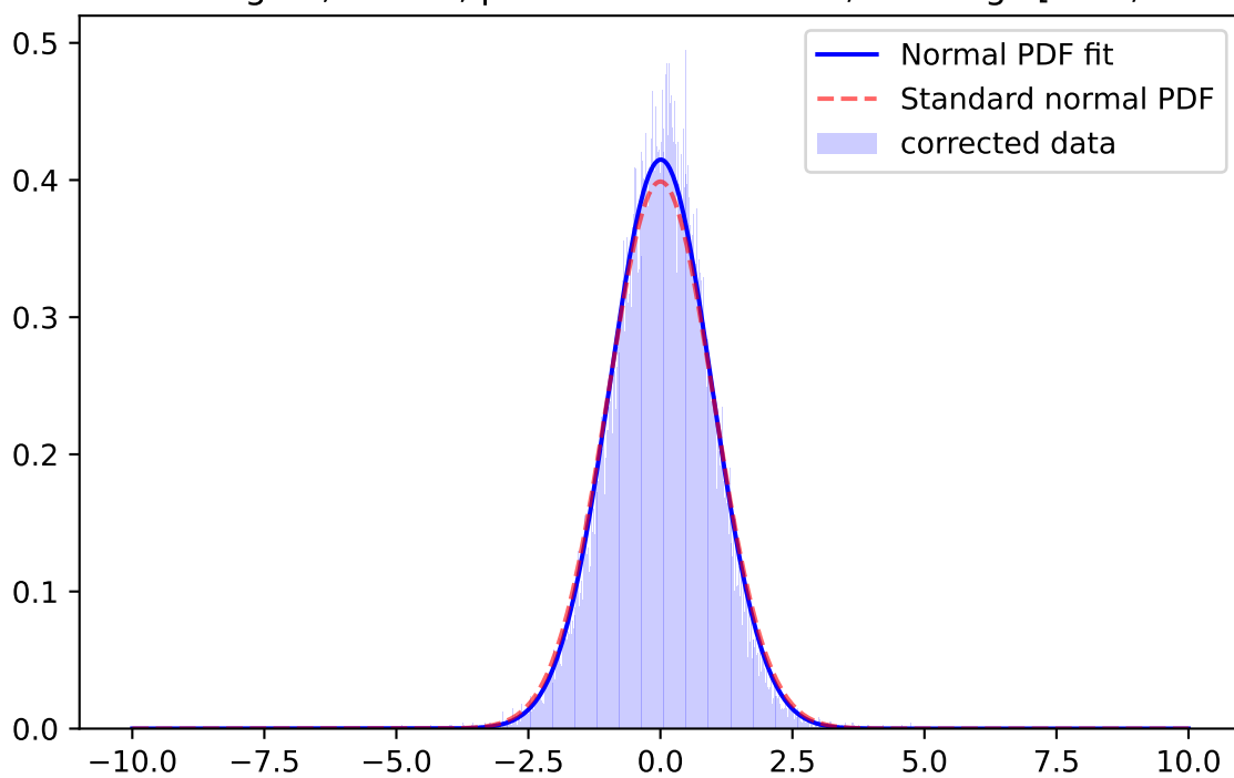
Whiten Signal, z-band, \mu=0.0135 \sigma=0.9696 ; for mag=[21.0; 21.5]
