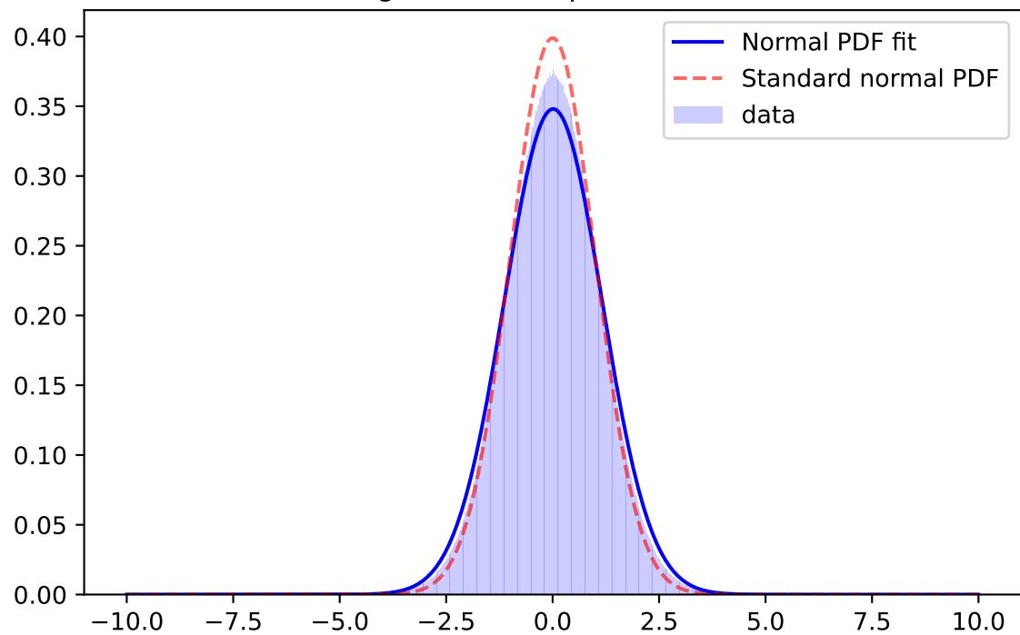
Whiten Signal, y-band, \mu=-0.0006 \sigma=1.1533
