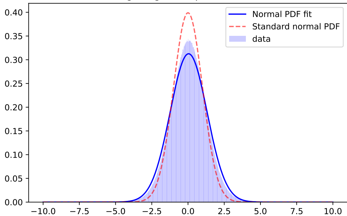
Whiten Signal, i-band, \mu=0.0127 \sigma=1.1462
