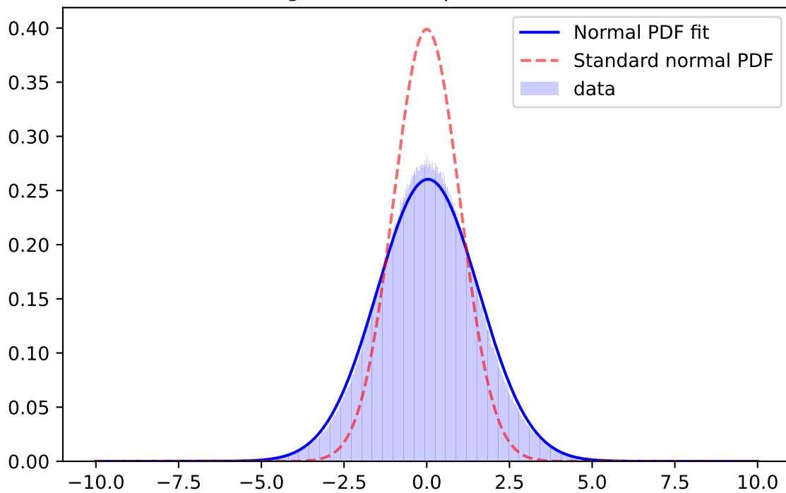
Whiten Signal, r-band, \mu=0.0311 \sigma=1.2545
