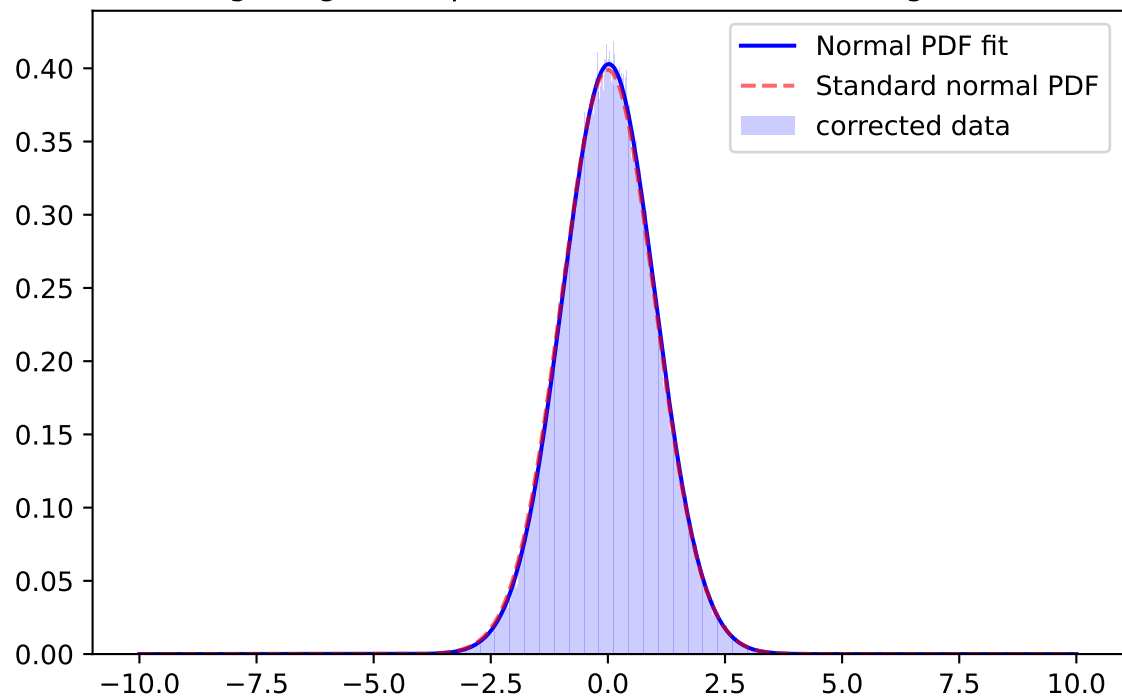
Whiten Signal, i-band, \mu=-0.0151 \sigma=0.9784 ; for mag=[25.0; 25.5]
