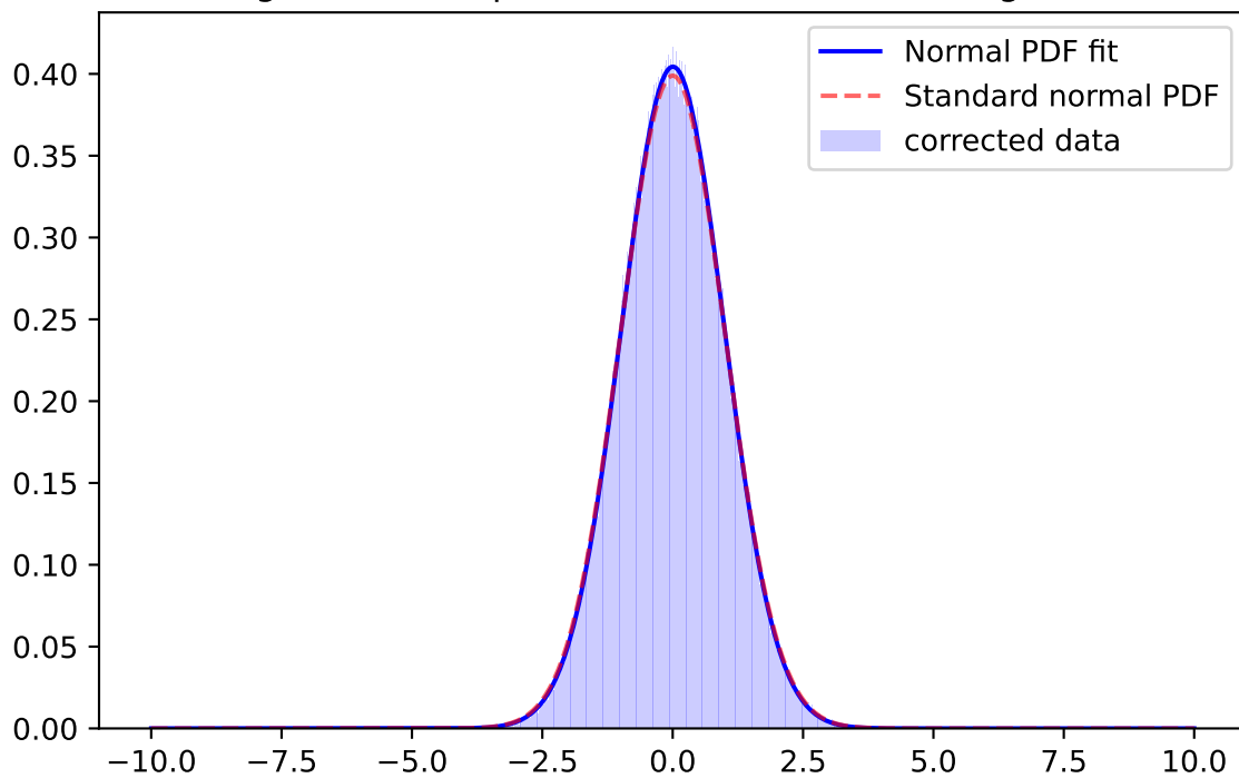
Whiten Signal, z-band, \mu=-0.0258 \sigma=0.9867 ; for mag=[25.0; 25.5]
