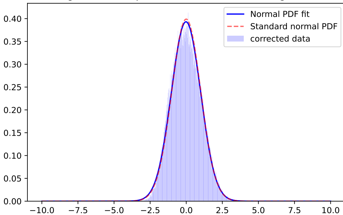
Whiten Signal, r-band, \mu=0.0036 \sigma=0.9864 ; for mag=[25.0; 25.5]
