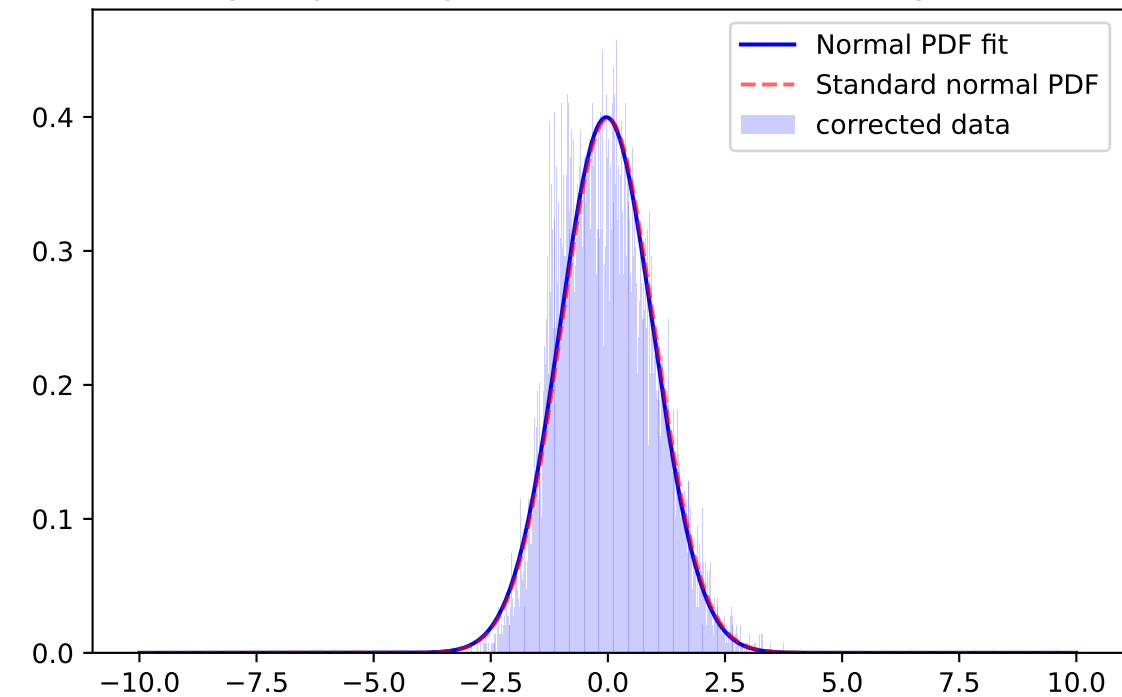
Whiten Signal, y-band, \mu=-0.0331 \sigma=0.9978 ; for mag=[25.0; 25.5]
