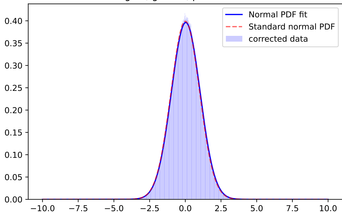
Whiten Signal, i-band, \mu=0.0013 \sigma=1.0018
