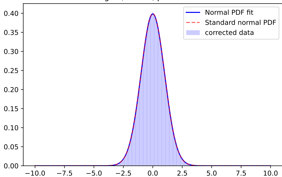
Whiten Signal, y-band, \mu=0.0057 \sigma=1.0104
