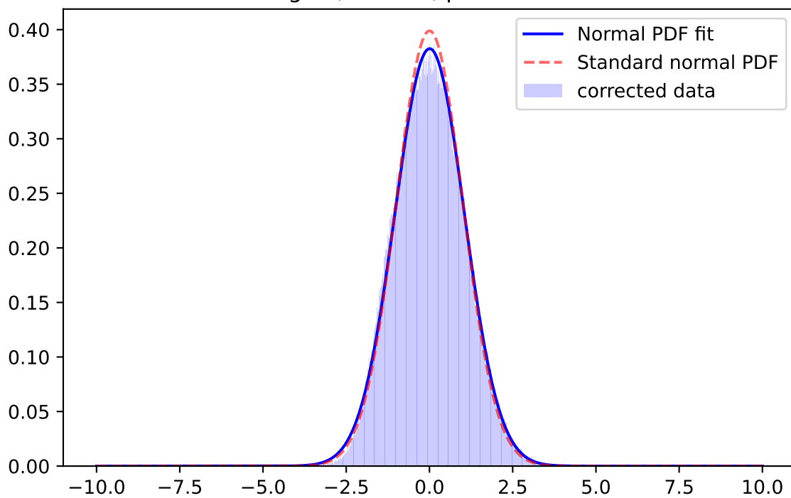
Whiten Signal, r-band, \mu=0.0223 \sigma=1.0150
