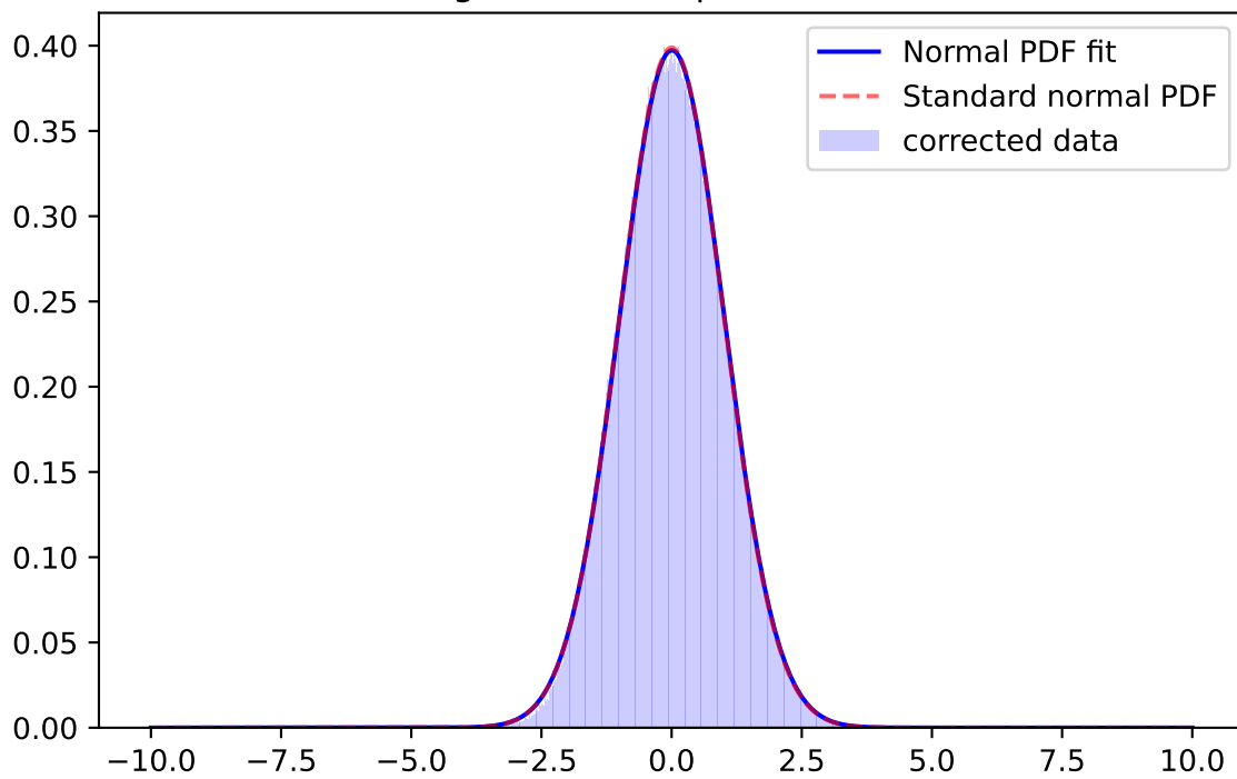
Whiten Signal, z-band, \mu=0.0053 \sigma=1.0041
