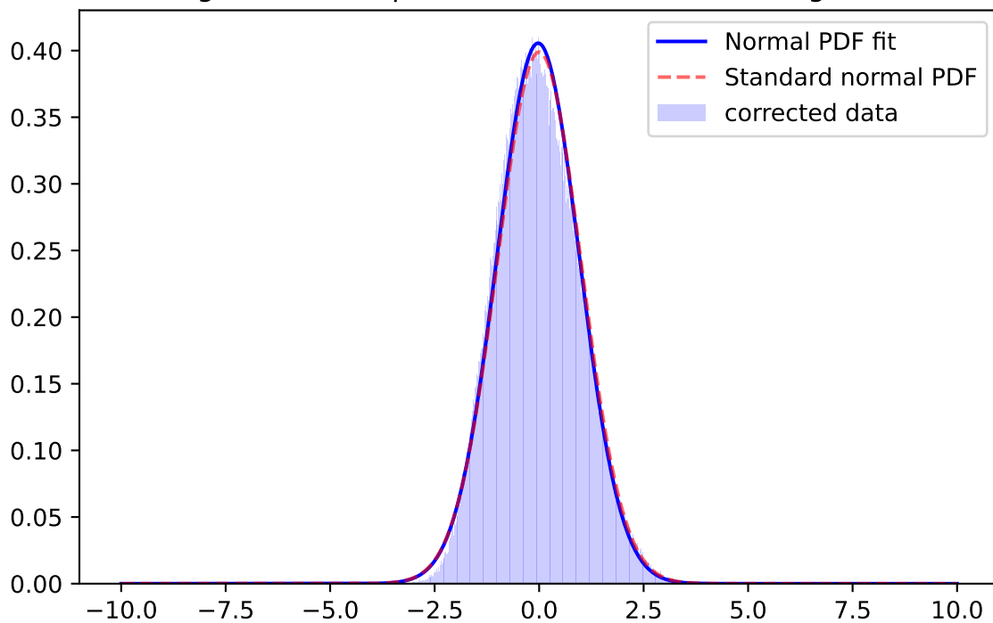
Whiten Signal, z-band, \mu=-0.0235 \sigma=0.9835 ; for mag=[25.0; 25.5]
