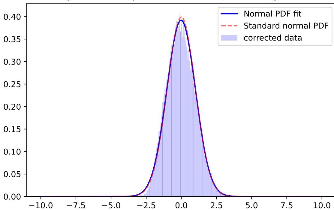
Whiten Signal, r-band, \mu=0.0040 \sigma=0.9898 ; for mag=[25.0; 25.5]
