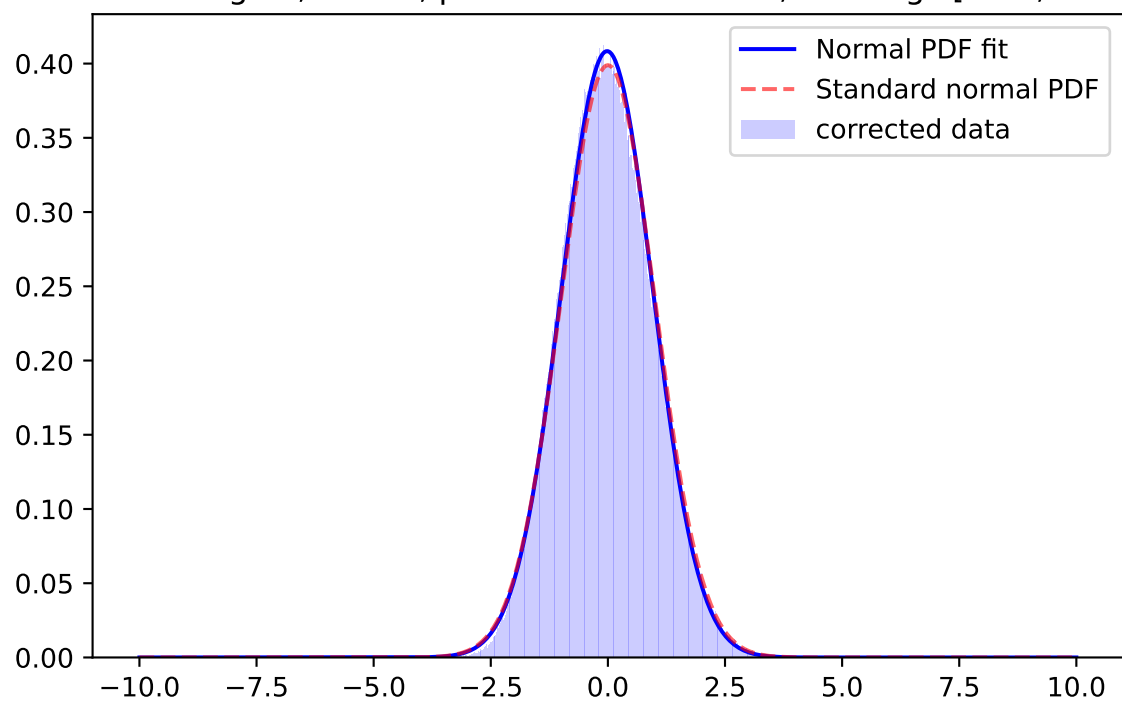
Whiten Signal, y-band, \mu=-0.0363 \sigma=0.9869 ; for mag=[25.0; 25.5]
