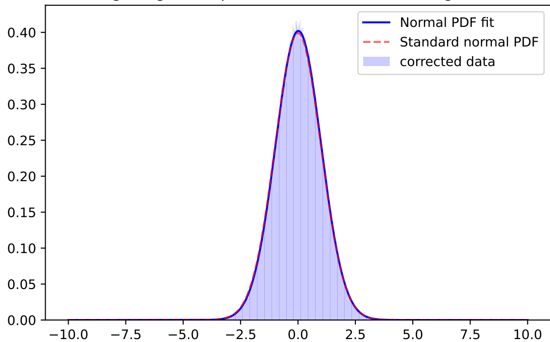
Whiten Signal, i-band, \mu=-0.0169 \sigma=0.9768 ; for mag=[25.0; 25.5]
