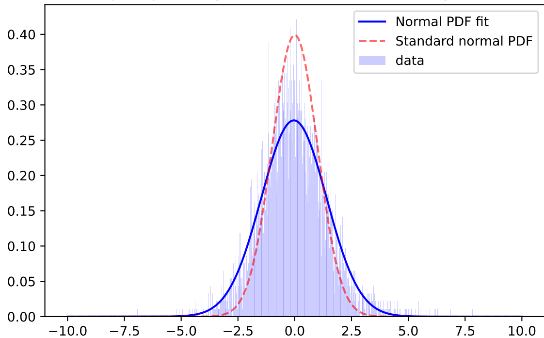
Whiten Signal, y-band, \mu=-0.0373 \sigma=1.4345 ; for mag=[18.0; 18.5]
