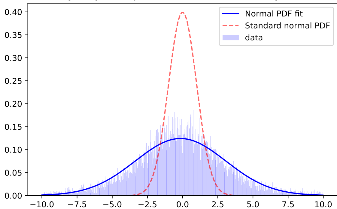
Whiten Signal, i-band, \mu=-0.0692 \sigma=3.2382 ; for mag=[18.0; 18.5]
