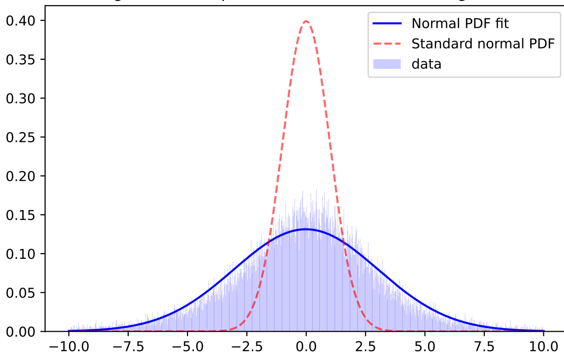
Whiten Signal, z-band, \mu=0.0043 \sigma=1.8782 ; for mag=[18.0; 18.5]
