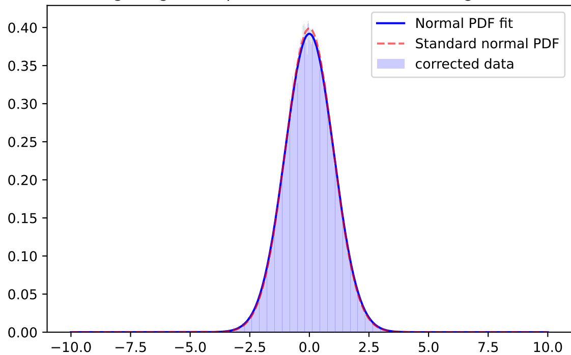
Whiten Signal, i-band, \mu=-0.0036 \sigma=1.0212 ; for mag=[25.0; 25.5]
