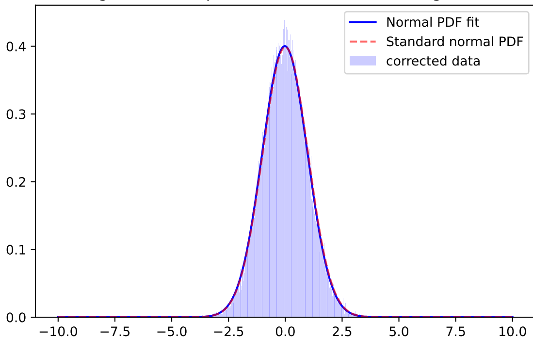
Whiten Signal, r-band, \mu=-0.0057 \sigma=1.0152 ; for mag=[25.0; 25.5]
