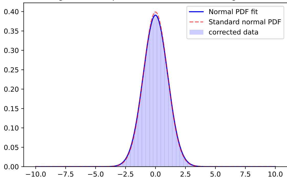
Whiten Signal, y-band, \mu=-0.0366 \sigma=0.9628 ; for mag=[25.0; 25.5]
