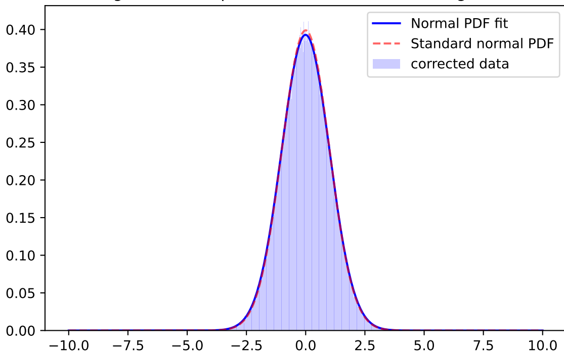
Whiten Signal, z-band, \mu=-0.0193 \sigma=0.9960 ; for mag=[25.0; 25.5]
