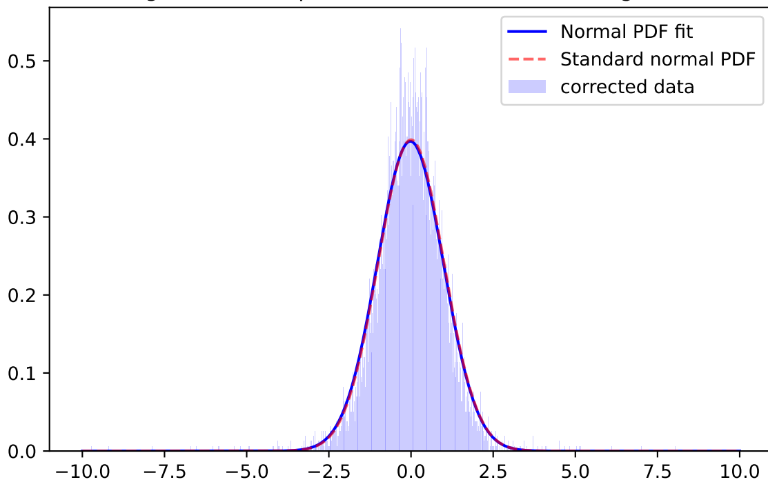
Whiten Signal, r-band, \mu=0.0048 \sigma=0.9781 ; for mag=[21.0; 21.5]
