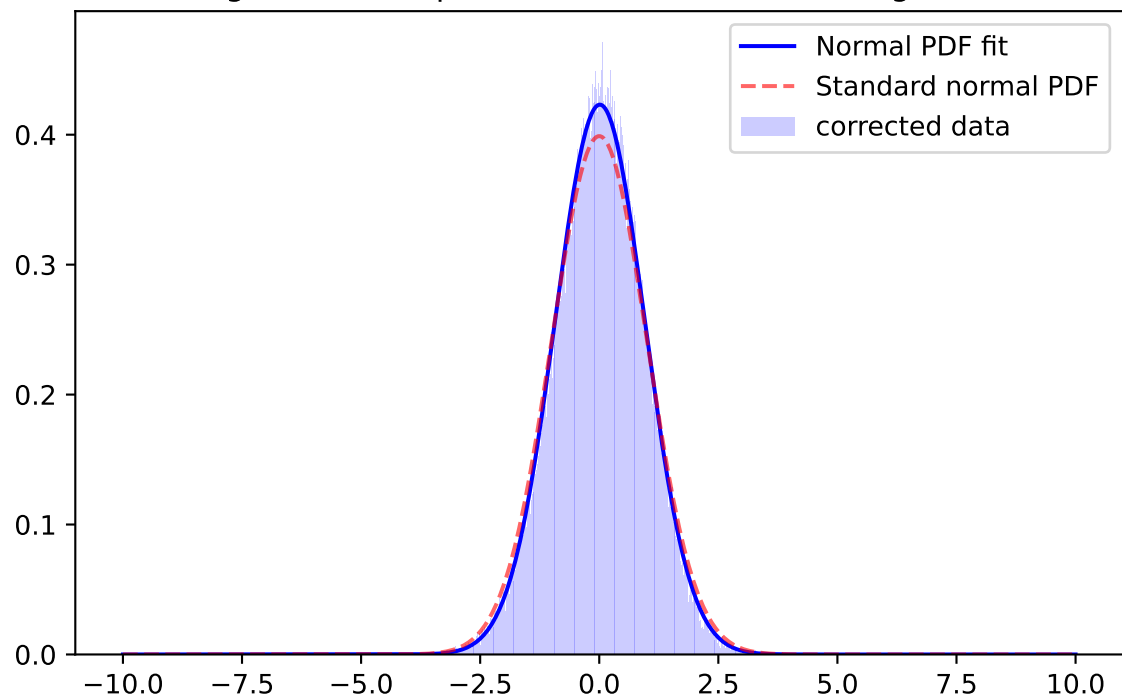
Whiten Signal, y-band, \mu=0.0368 \sigma=0.9467 ; for mag=[21.0; 21.5]
