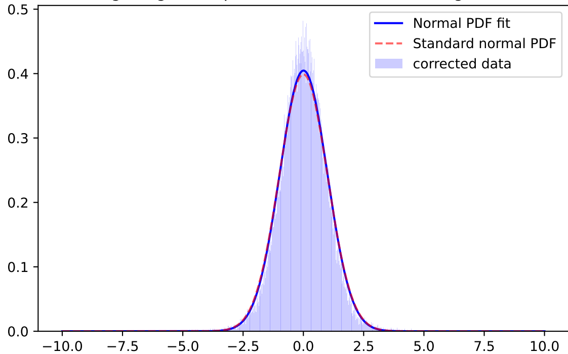
Whiten Signal, i-band, \mu=0.0124 \sigma=0.9427 ; for mag=[21.0; 21.5]
