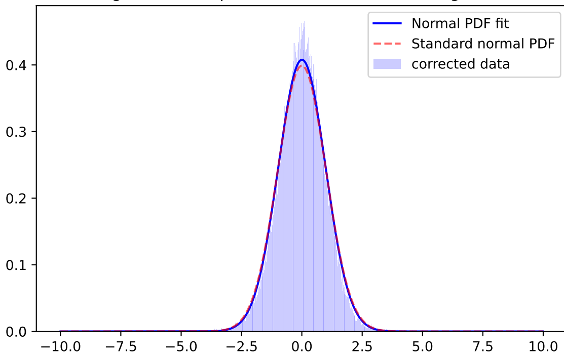
Whiten Signal, z-band, \mu=0.0142 \sigma=0.9624 ; for mag=[21.0; 21.5]
